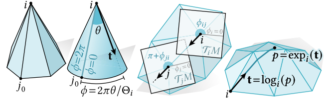
Fig. 6. Notation and conventions for tangent vectors (left), parallel transport (center), and the logarithmic/exponential maps (right).
