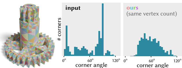
Fig. 13. Even for an identical vertex count, refining then coarsening yields higher quality elements, as quantified by histograms of corner angles \theta_{ijk}^j .
