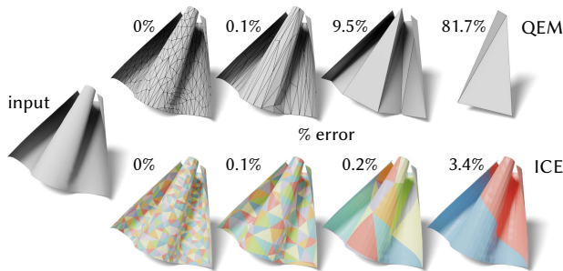
Fig. 19. On surfaces with small intrinsic curvature, such as a developable surface obtained from [Rabinovich et al. 2018], we achieve dramatically lower error in surface area compared to extrinsic methods like QEM.
