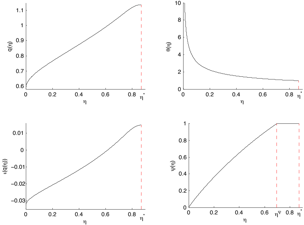
Figure 1: Equilibrium functions q(\eta) , \theta(\eta) , \iota(q(\eta)) and \psi(\eta) .
