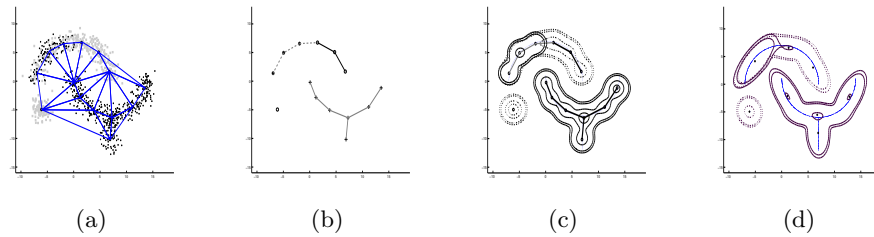
Fig. 1: Principle of the Supervised Generative Graph. We drawn 1000 data from the four principal manifolds (drawn figure 1 (d)) corrupted with an additive gaussian noise with variance \sigma^2 = 0.81 . First and second classes are respectively represented by 'black +' and 'grey o'. The top left quarter-circle is mixed '+' and 'o', the right one and the point are 'o' and the Y-shaped is '+'. (a) The prototypes are located with a GGM (identical variances) and the EM algorithm. They are connected with edges from the Delaunay graph. (b) The optimal SGGG obtained after optimization of the likelihood according to \sigma , \underline{\beta} and \underline{\pi} and pruning of the edges associated to a null or almost null prior. The edges representing only one class (resp. several classes), i.e. \max_c(\beta_{c_j}^d) = 1 are in black (resp. dotted) lines. (c-d) Iso-density curves at values (0.0005, 0.001, 0.05, 0.01) for each class given by the SGGG and the best GGM (free covariances) which has been selected with the appropriate BIC criterion. The estimated variance of the noise \hat{\sigma}^2 by the SGGG is equal to 0.98. The variance is over estimated because non linear manifolds are approximated by piecewise linear manifolds. In order to evaluate the accuracy of the generative model SGGG, we estimated the Normalized Negative Loglikelihood (NNL) on an independent sample of 5000 data for both models : NNL_{SGGG} = 5,0154 and NNL_{GMM} = 5,5447 .
