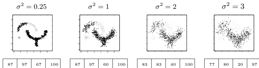
Fig. 2: SGGG with various noise conditions: The noise variances are set to \sigma^2 = 0.25, 1, 2 and 3 . The figures represent one data set over the 30 different data set which have been randomly drawn for each noise value. The results are given in percent and represent the number of models which have correctly modeled the four principal manifolds (the top-left quarter-circle, the top-right quarter-circle, the 'Y-shaped' and the point).
