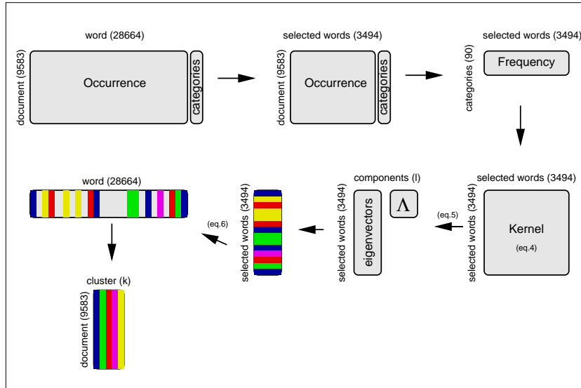
Fig. 1: The scheme of the algorithm.
