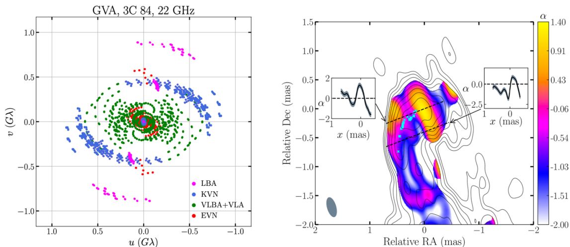
Spectral index distribution of 3C 84 derived from the images obtained with the GVA (a global array of telescopes including the EVN, KVN, VLBA, VLA and the LBA, see uv-coverage on the left). The inverted spectrum at the edge of the inner jet is likely due to interaction with a dense cold ambient medium, which is believed to contribute to the observed deflection of the jet. Detailed imaging of complex structures like this requires efforts on global scales. Park et al. (2024), A&A, 685, A115
