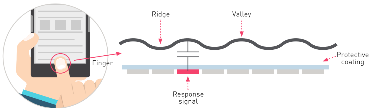
Figure 24. Capacitive sensing principle: The measured capacitances varies with the ridges and valleys of the fingerprint.
