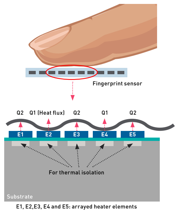
Figure 30. Principle of active thermal fingerprint detection
