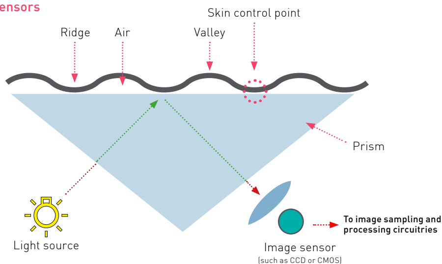
Figure 23. Working principle of an optical fingerprint sensor
