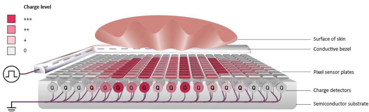
Figure 25. Active capacitive measurement with an active bezel charging the finger
