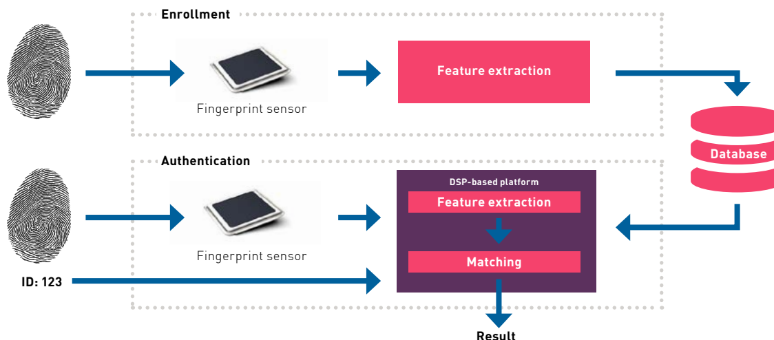
Figure 21. Block diagram of an automated fingerprint recognition system
