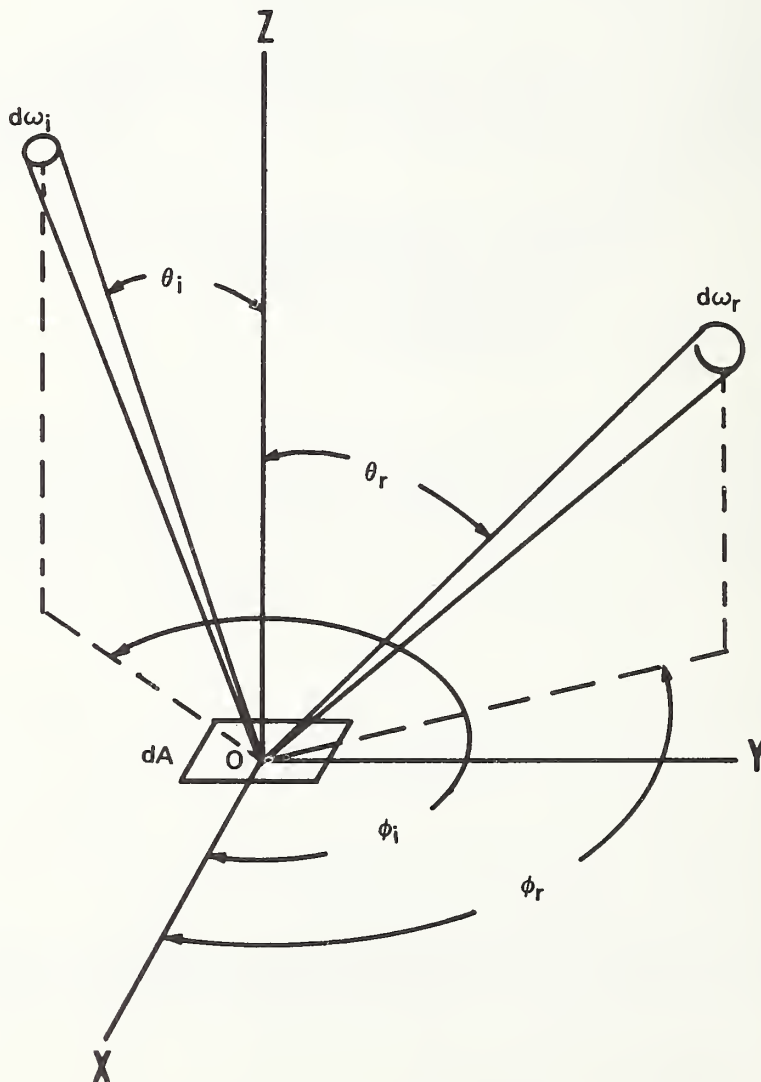
FIGURE 2. Geometry of incident and reflected elementary beams. (Z-Axis is chosen along the normal to the surface element dA at 0.) (adapted from [10]).
