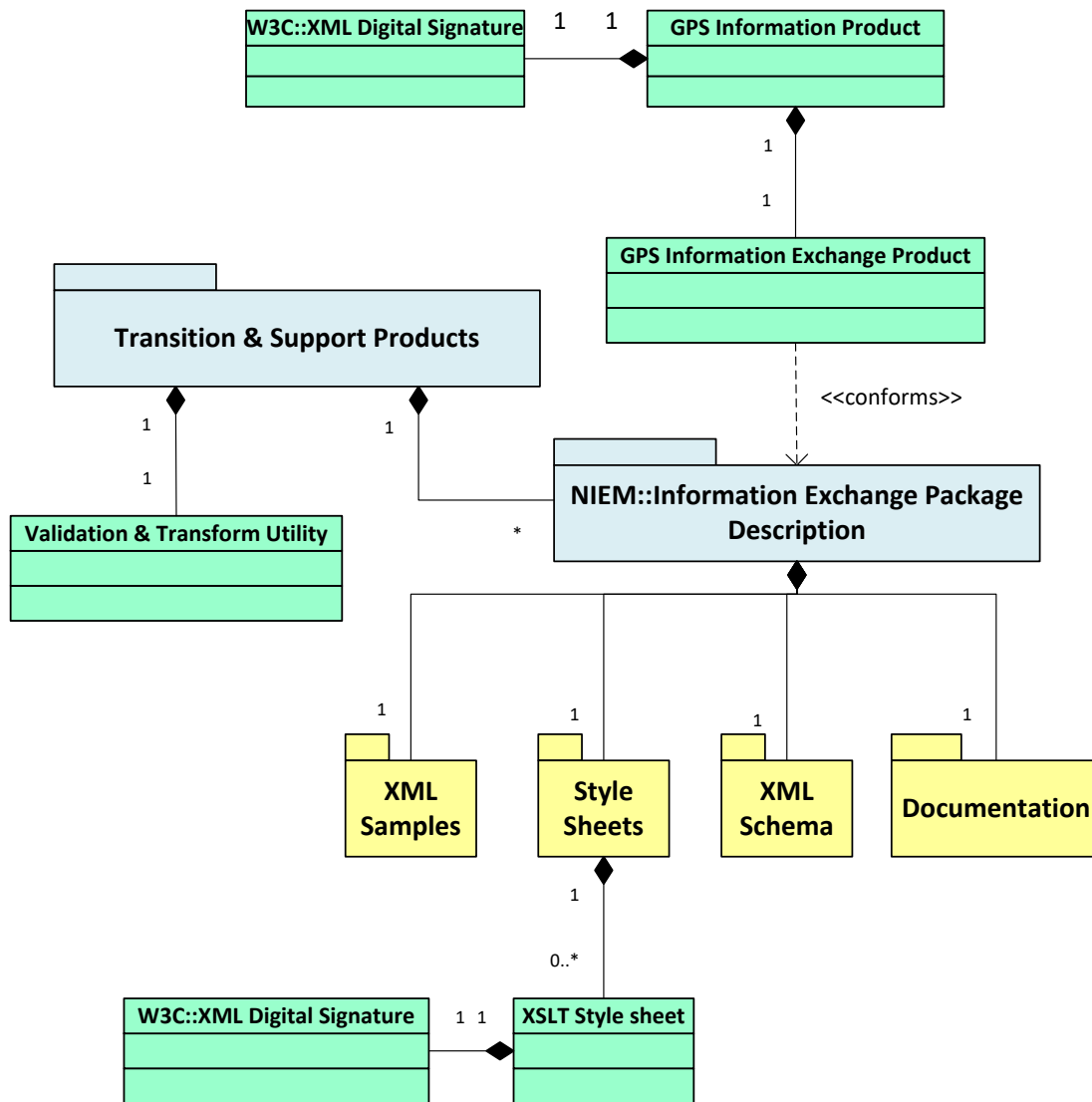
Figure 3-3 High Level GPS Product Ontology
