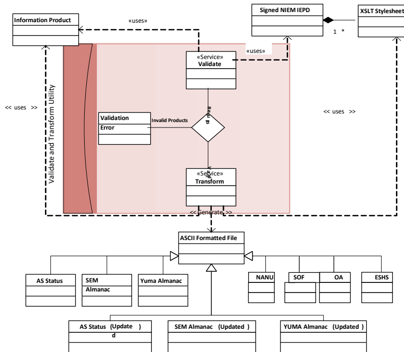
Figure 3-4 Validate and Transform Utility Ontology
