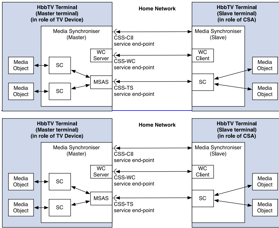
Figure 22: Relationship between the HbbTV® MediaSynchroniser and MSAS, SC, WC Server and WC Client elementary functions and protocol service endpoints
