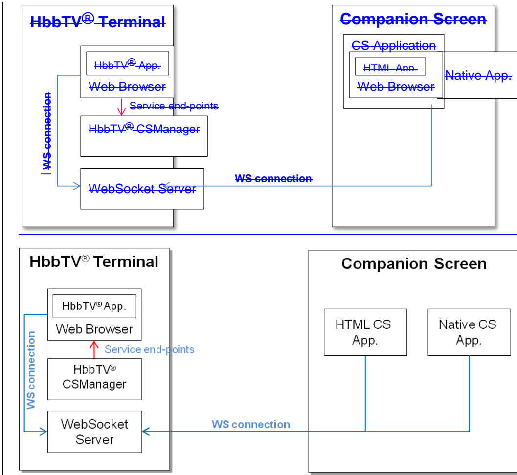
Figure 32: Architecture for application to application communication
