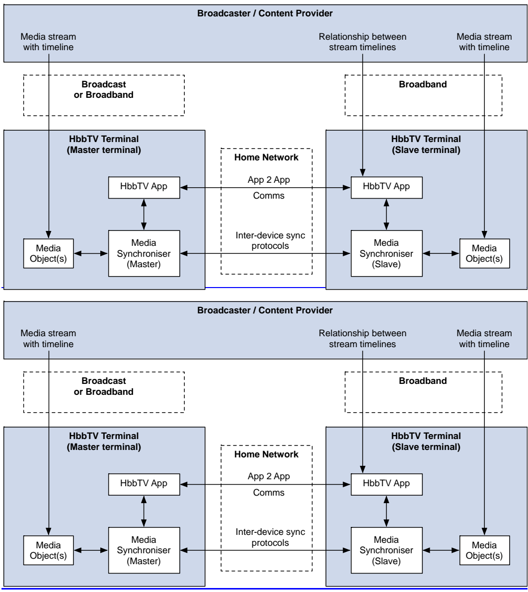
Figure 20: Relationship between MediaSynchroniser object and HbbTV® application for inter-device synchronization with a slave terminal
