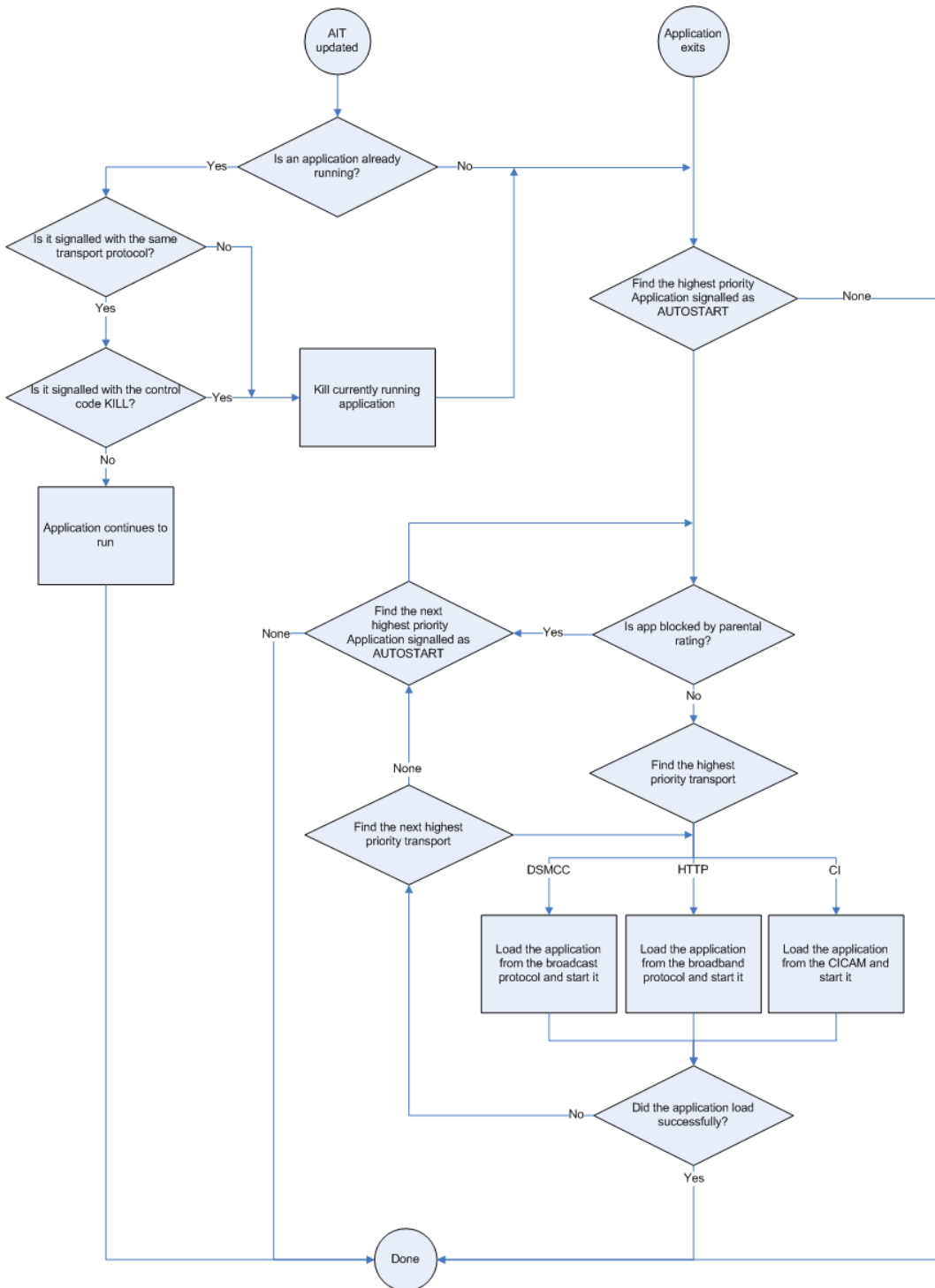
Figure 14: Behaviour while a broadcast service is selected
