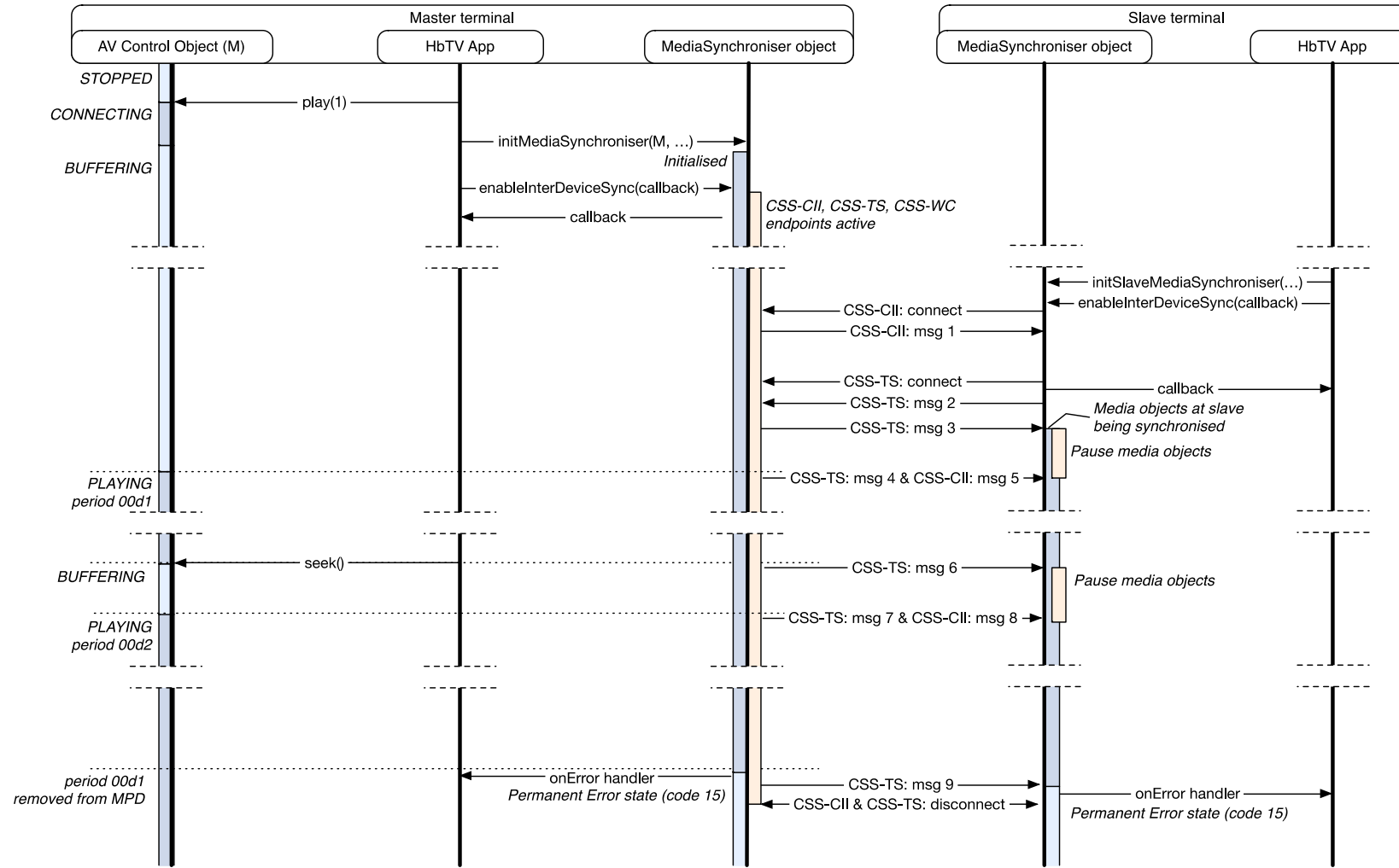
Figure 28: Inter-device synchronization sequence diagram where master media is an AVAV Control object playing an MPEG DASH presentation
