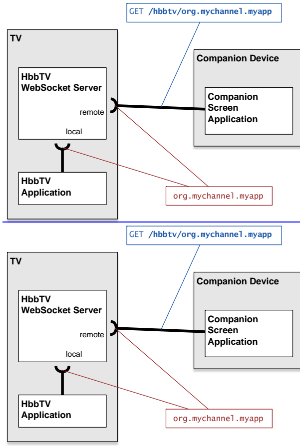
Figure 37: Two waiting connections that will be paired by the TV
