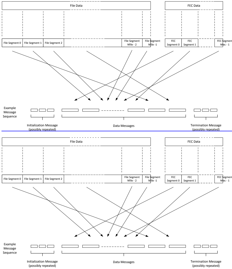
Figure H.1: FDP message sequence
