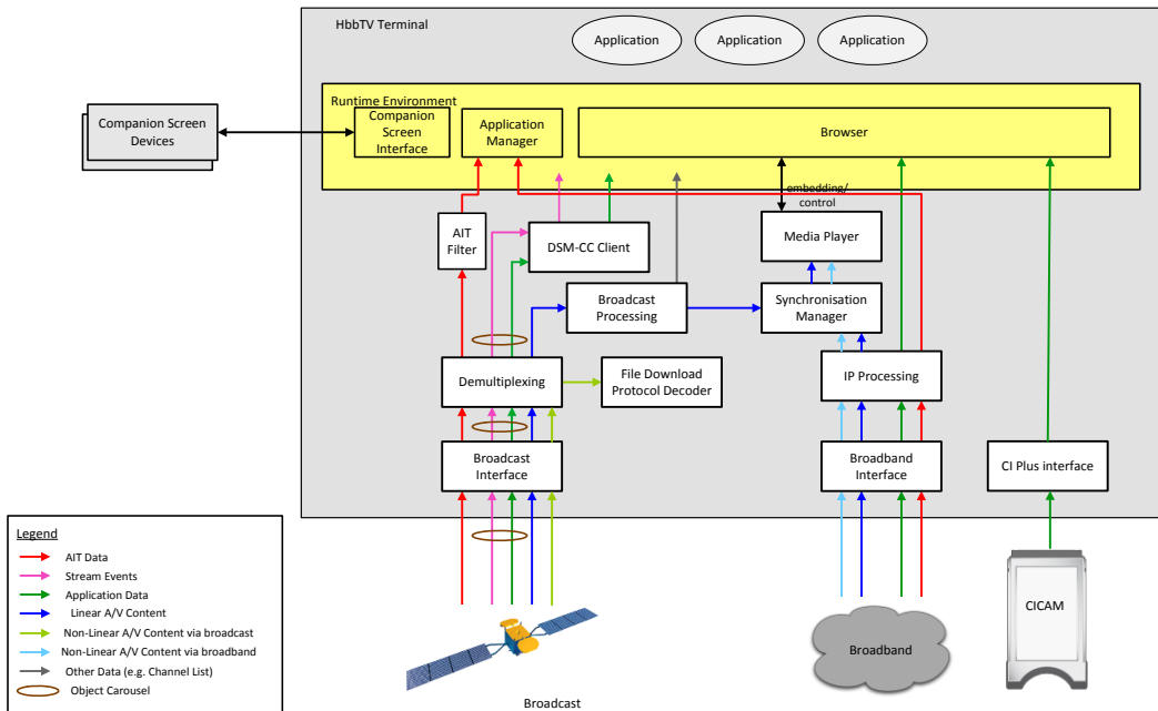
Figure 2: Functional components of a hybrid terminal
