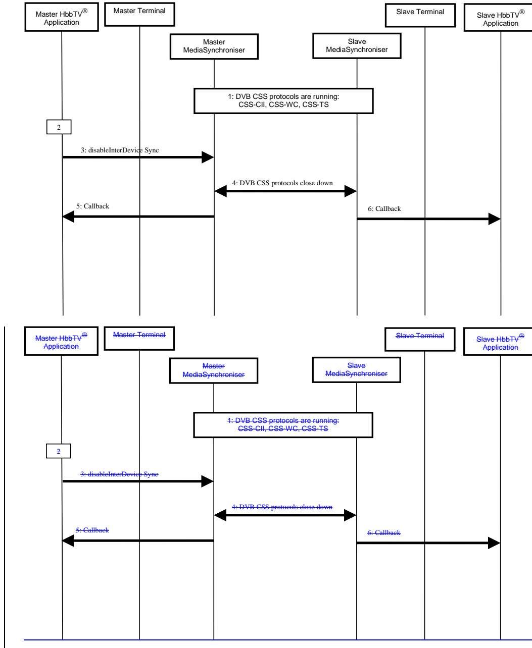
Figure 26: Termination of inter-device timeline synchronization
