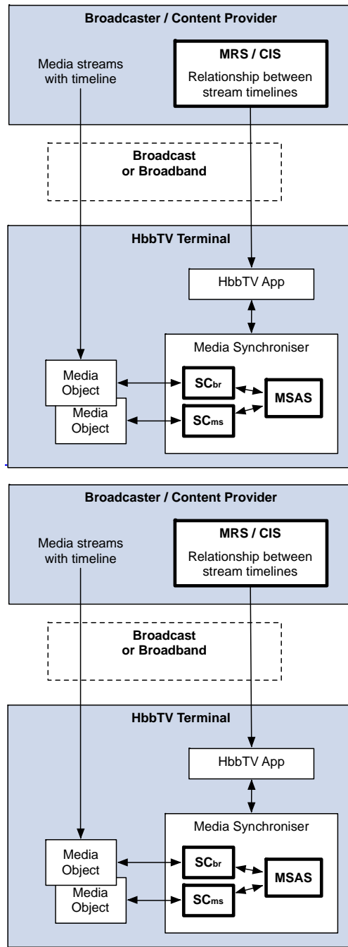
Figure 18: Basic mapping of media synchronization architecture for multi-stream synchronization
