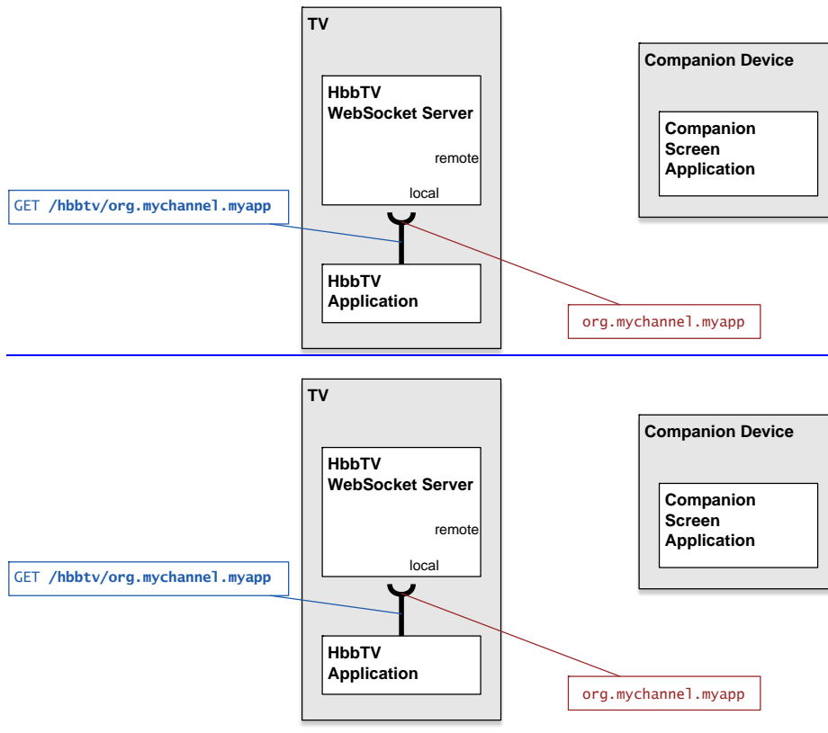
Figure 35: A waiting connection for application to application communication
