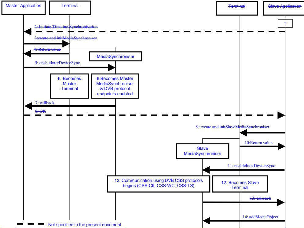
Figure 24: Initiation of inter-device timeline synchronization
