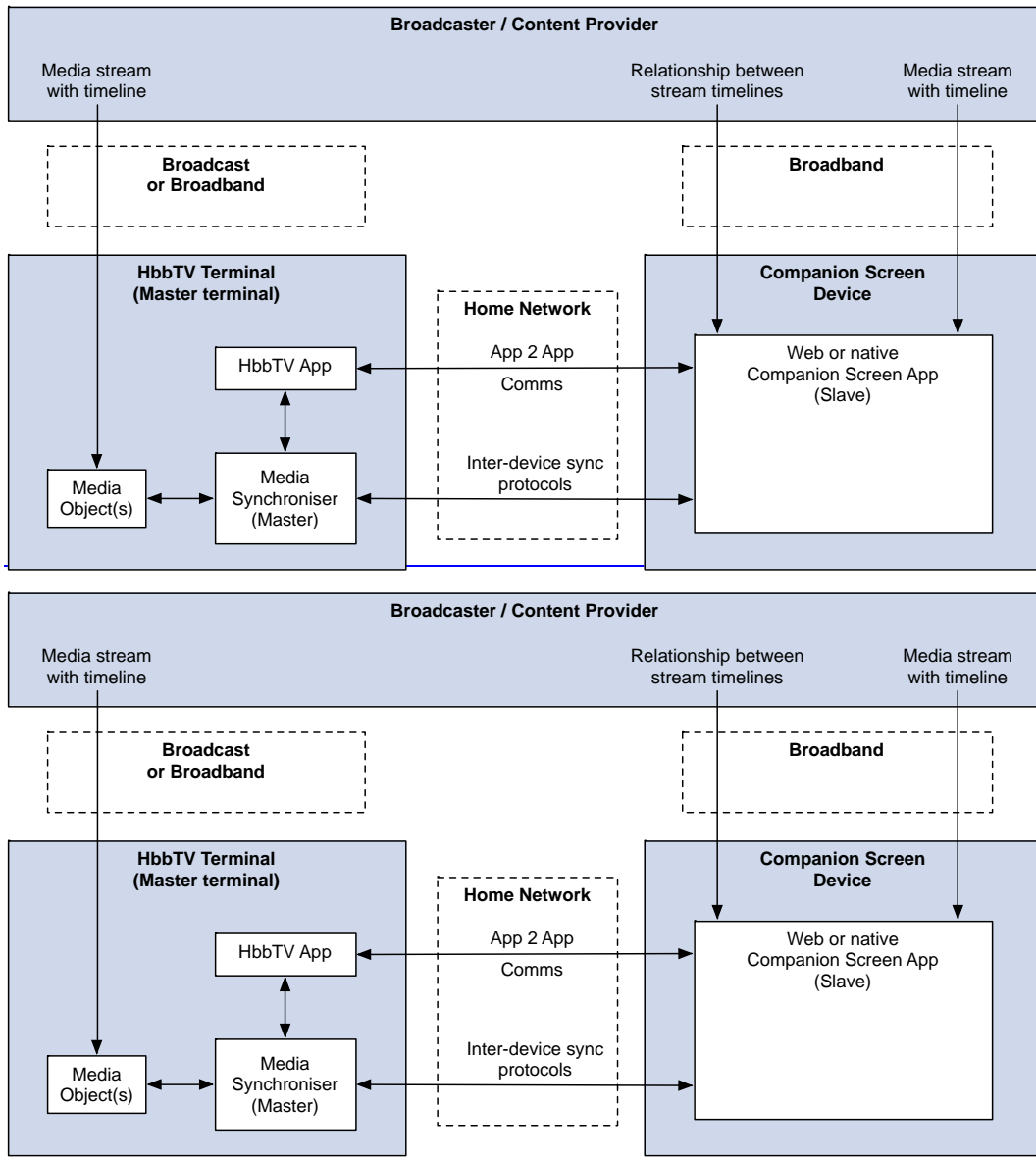
Figure 19: Relationship between MediaSynchroniser object and HbbTV® application for inter-device synchronization with a CSA
