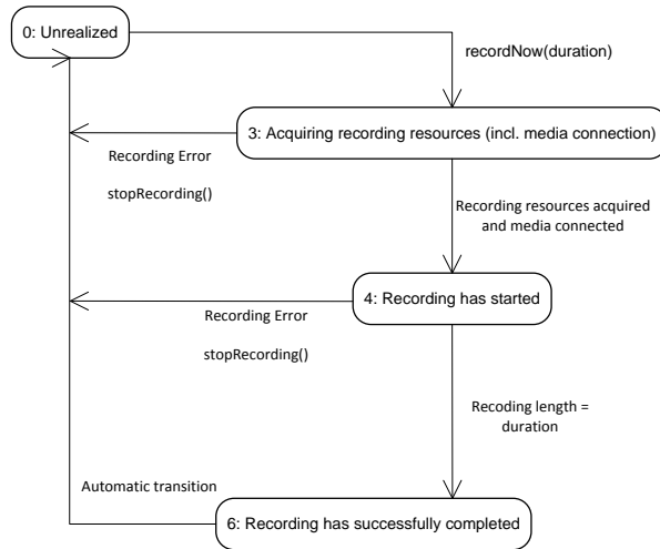
Figure 38 the AV: PVR States for recordNow using video/broadcast (normative)
