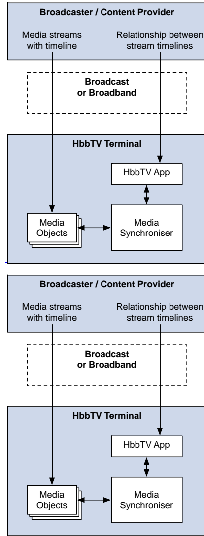
Figure 17: Relationship between MediaSynchroniser object and HbbTV ® application for multi-stream synchronization
