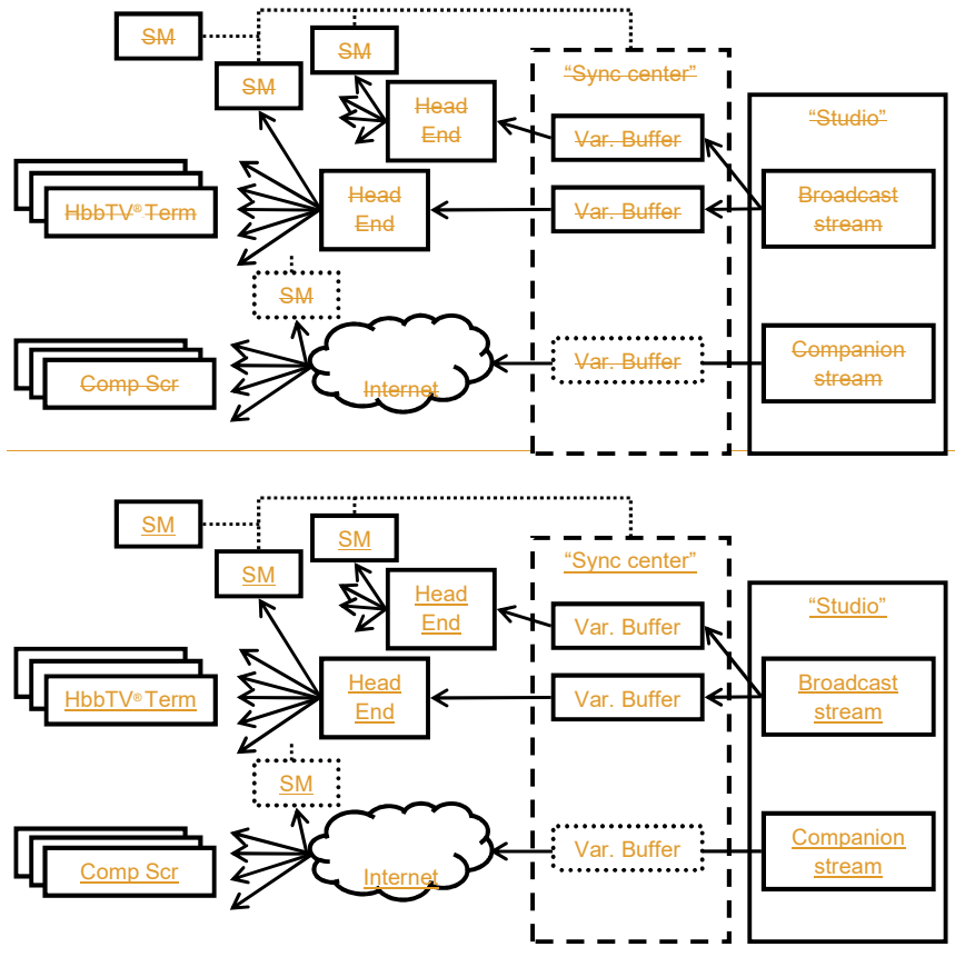
Figure G.1: Architecture for delay management and equalisation
