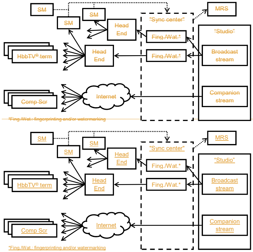
Figure G.2: Architecture for managing multiple content timelines
