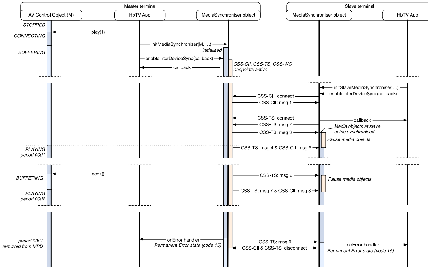
Figure 28: Inter-device synchronization sequence diagram where master media is an A/V Control object playing an MPEG DASH presentation
