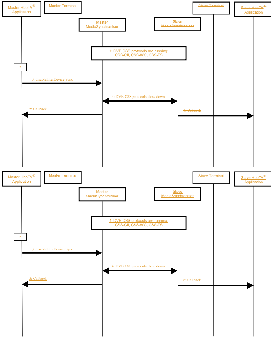
Figure 26: Termination of inter-device timeline synchronization
