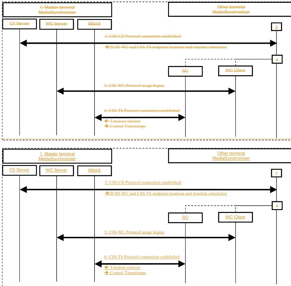
Figure 25: Protocol interactions for inter-device timeline synchronization
