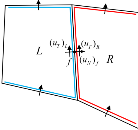
Figure 1. Double-C stencil used for computing the face tangential velocity.
