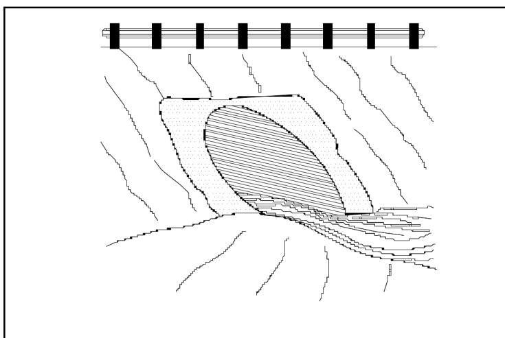
Culvert Inlet Mitered to Conform to Slope
