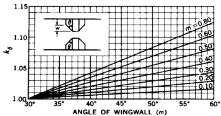
b) Wingwall adjustment factor.
