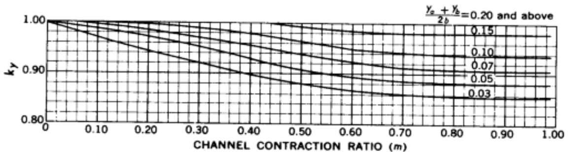
b) Average depth adjustment factor.
