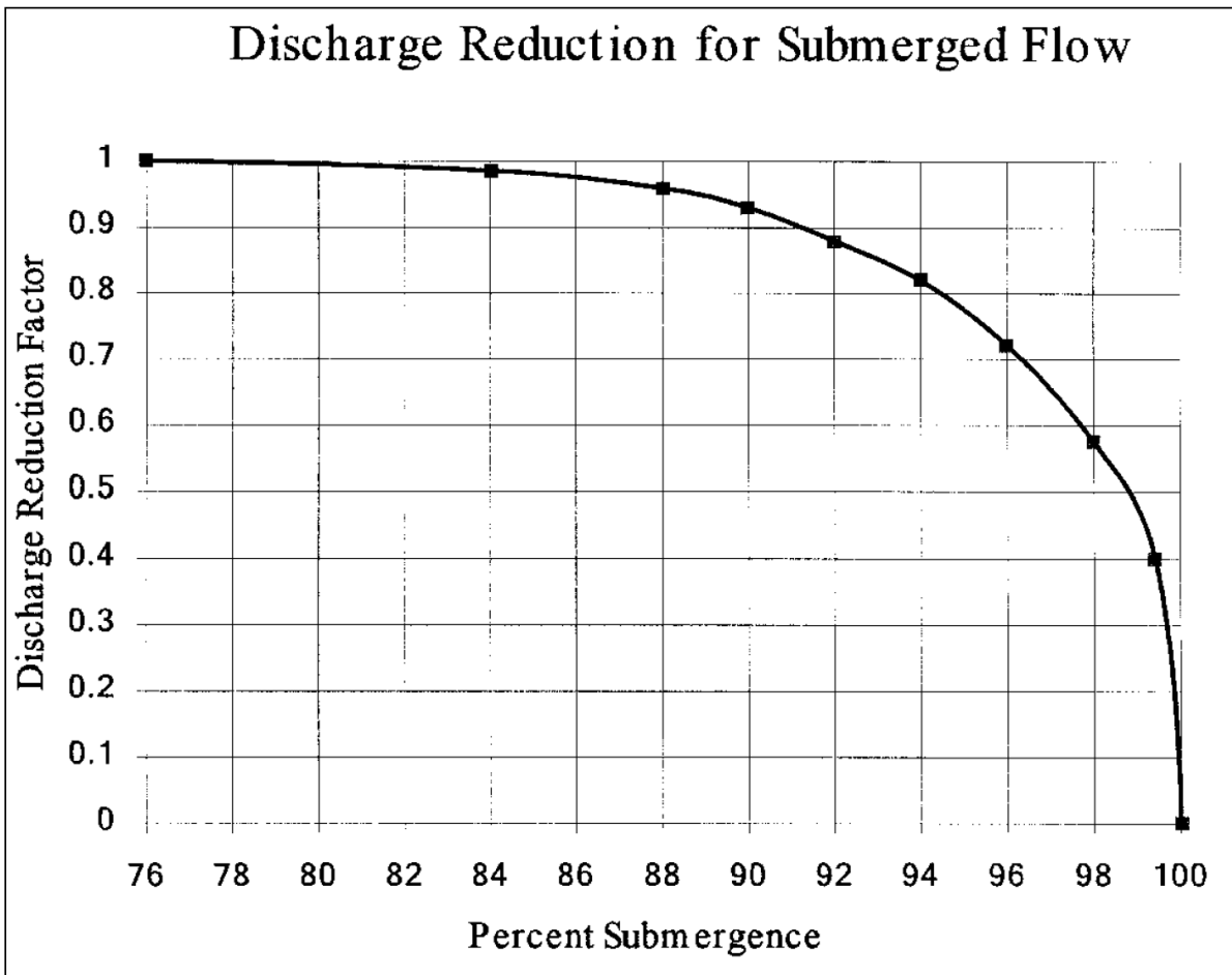
Factor for reducing weir flow for submergence
