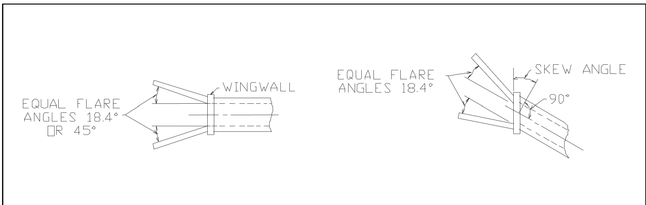
Non-Offset Flared Wingwalls (Chart 12)
