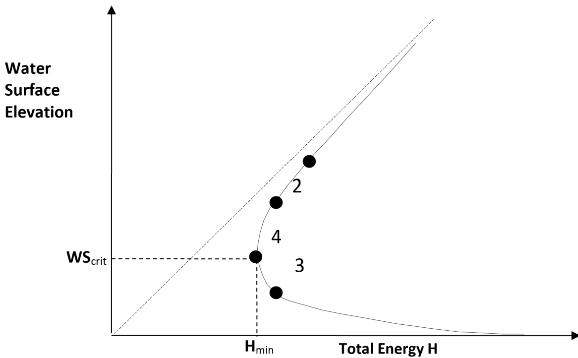
Energy vs. Water Surface Elevation Diagram
