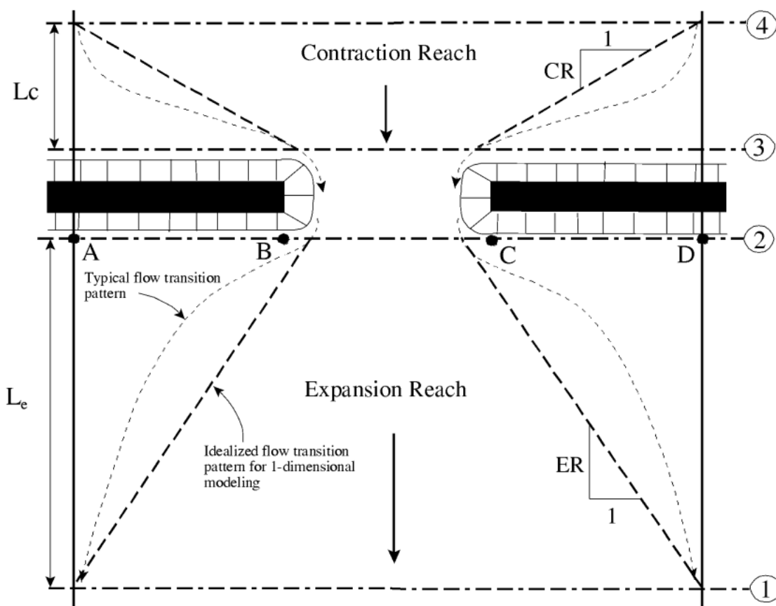
Figure 5-1 Cross Section Locations at a Bridge
