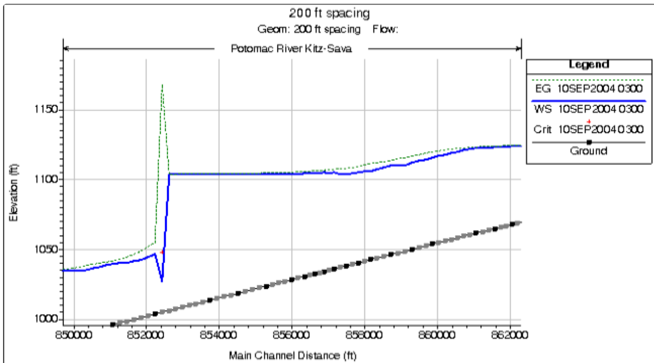
Example Model Instability due to Very Short Cross Section Spacing.
