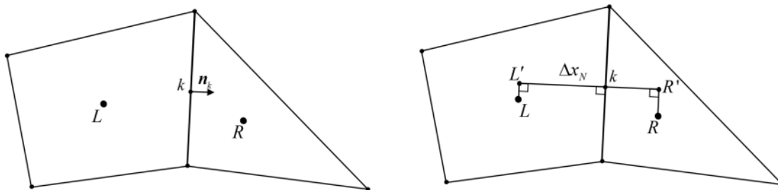
Cell Directional Derivatives
