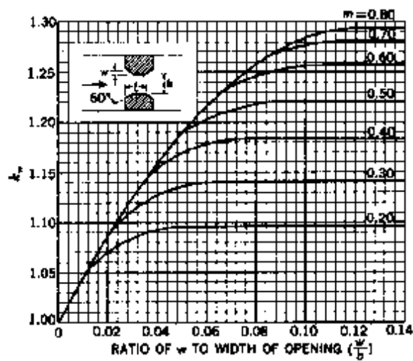
c) 60° wingwalls.
