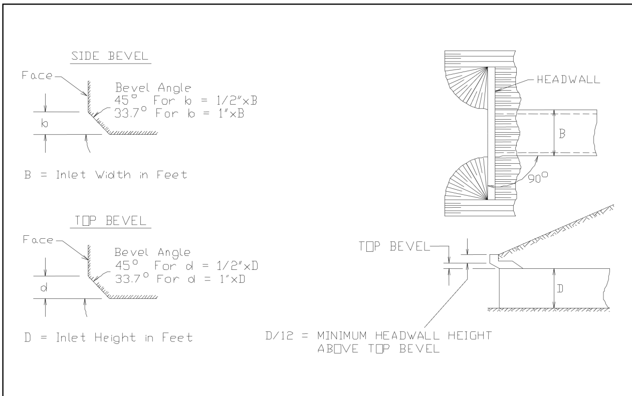
Inlet Side and Top Edge Bevel with Ninety Degree Headwall (Chart 10)
