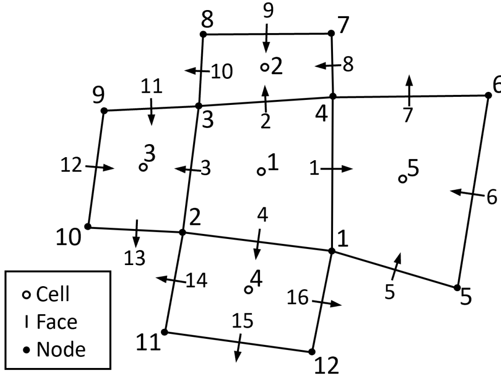
Figure 1. Example mesh with cell, face, and node numbering.
