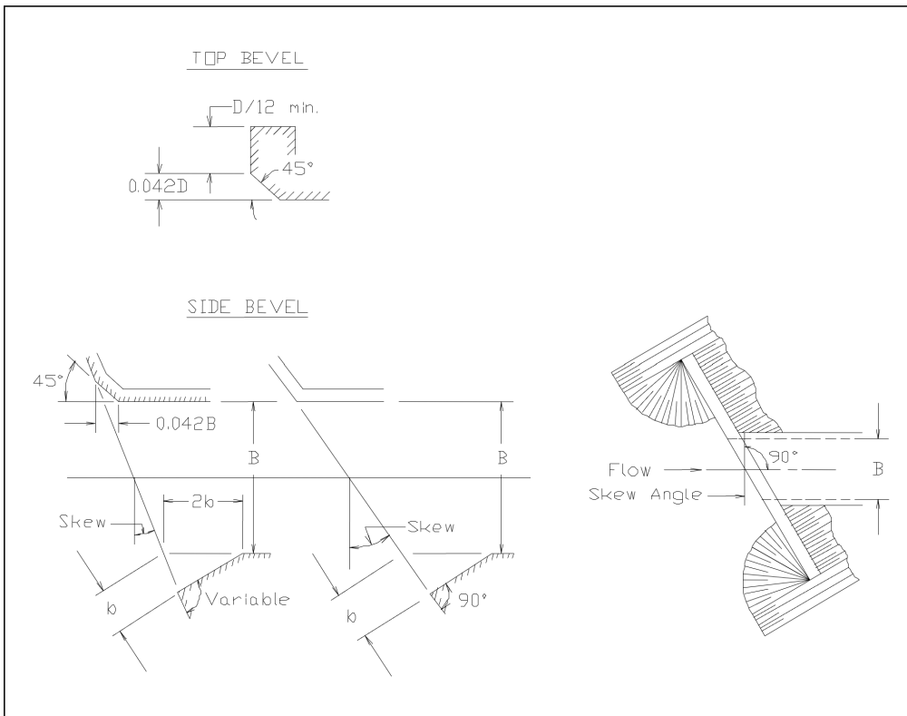
Inlet Side and Top Edge Bevel with Skewed Headwall (Chart 11)
