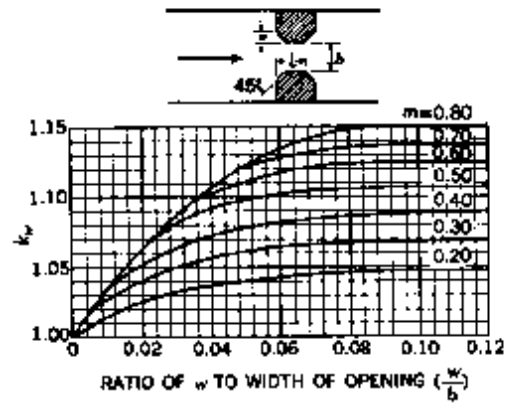
b) 45° wingwalls.
