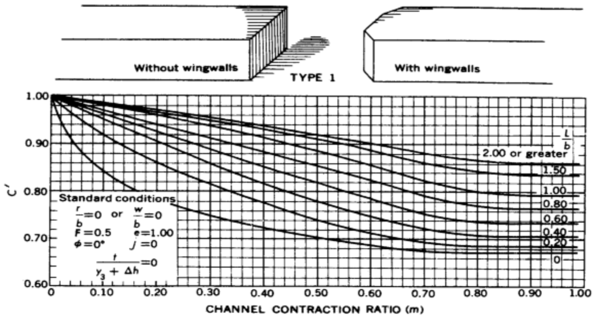
a) Base coefficient of discharge.
