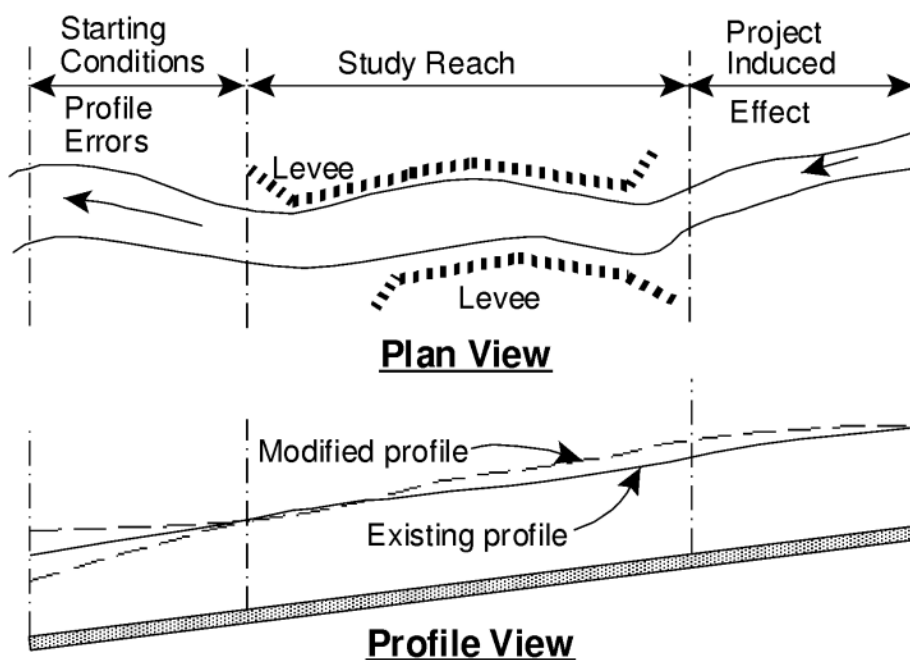
Example Study Limit Determination
