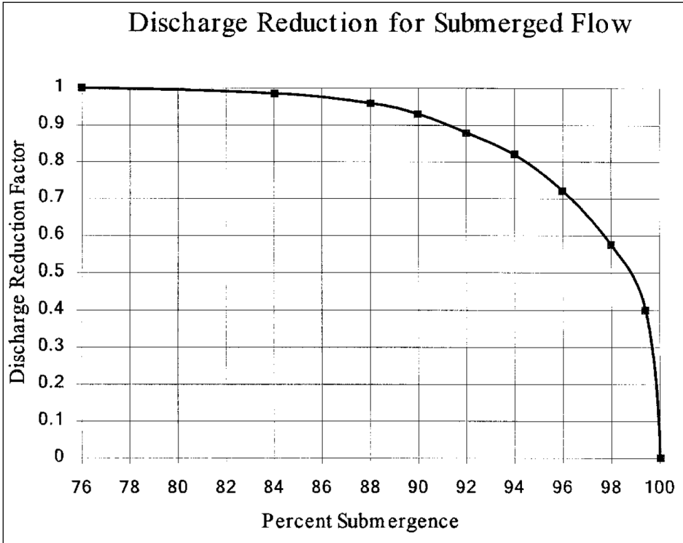
Factor for reducing weir flow for submergence
