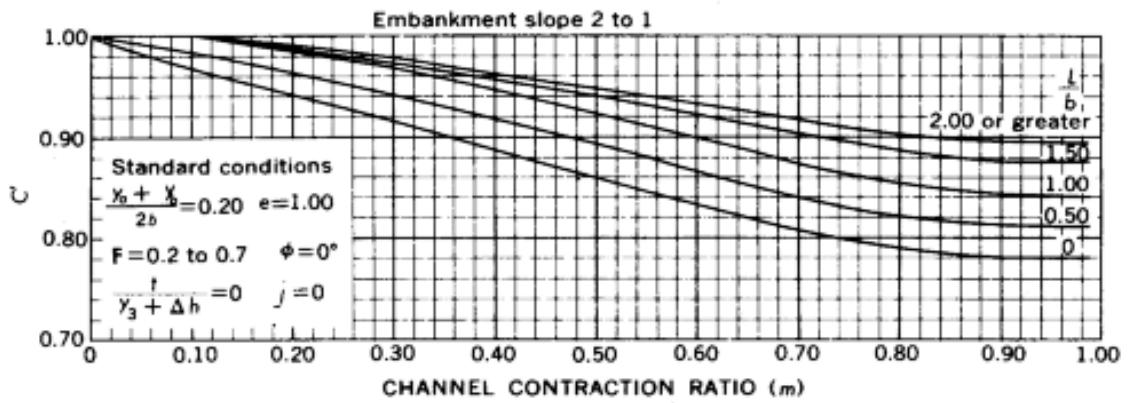
a) Base coefficient of discharge.
