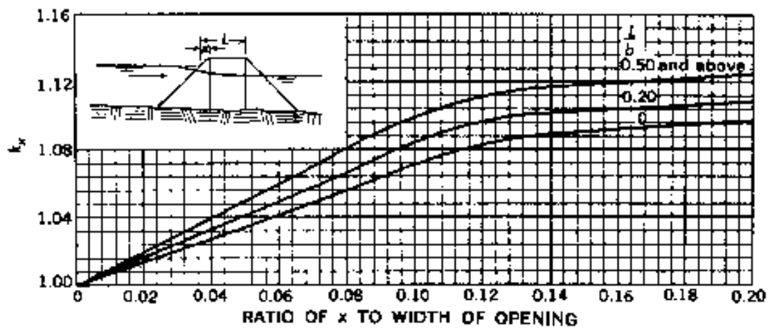
b) Unwetted abutment adjustment factor.
