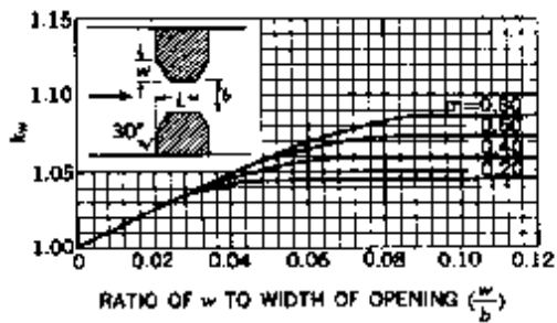
a) 30° wingwalls.
