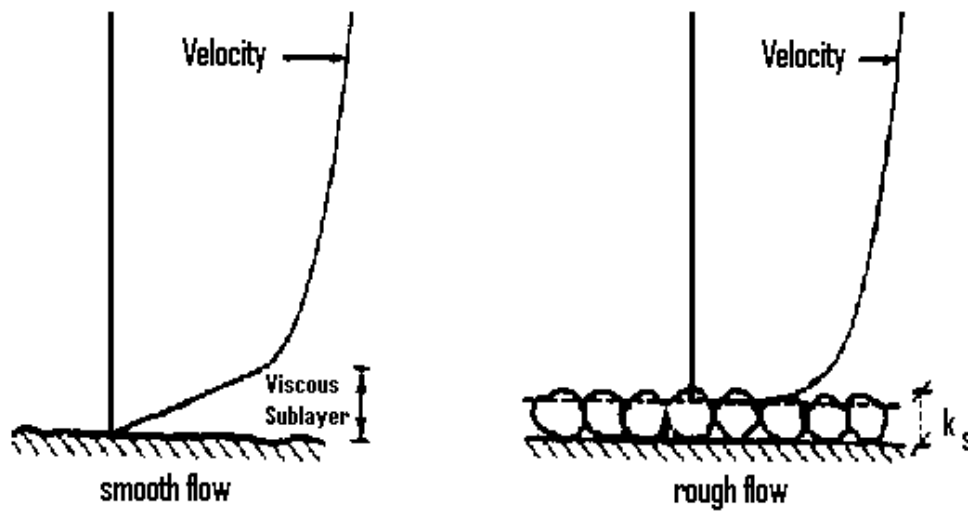
Velocity Distribution in Smooth and Rough Flow (Van Rijn, 1993)
