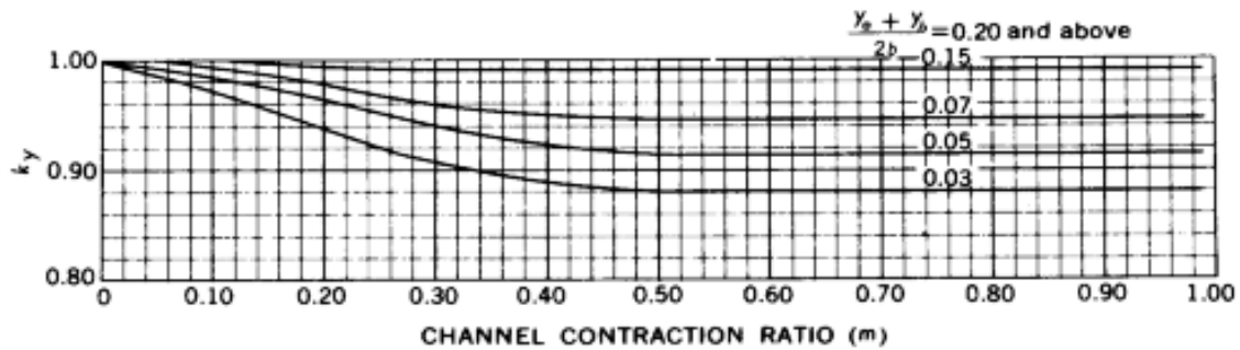
b) Average depth adjustment factor.
