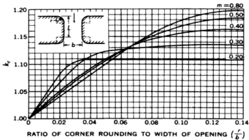
c) Corner rounding adjustment factor.
