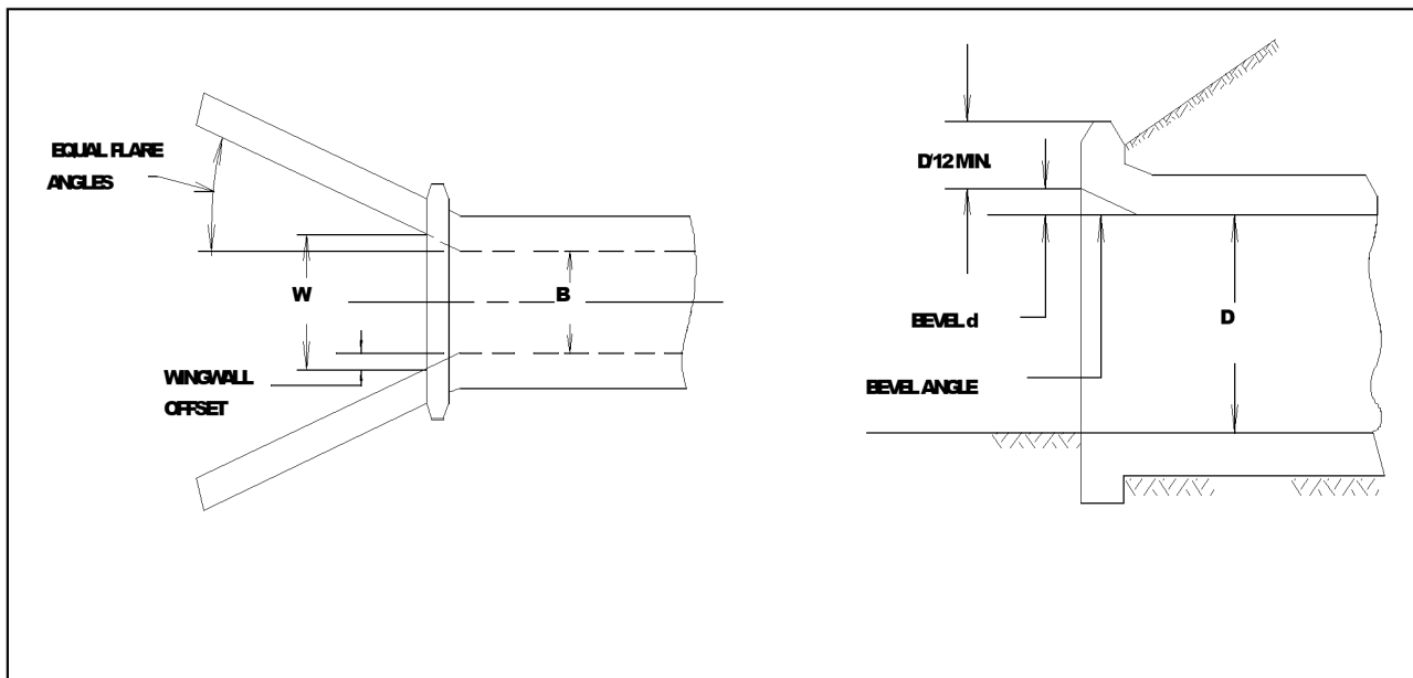
Offset Flared Wingwalls (Chart 13)
