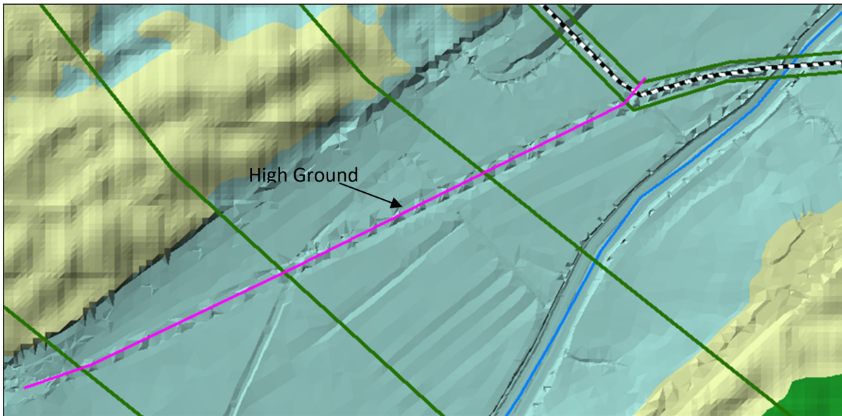
High ground (road or levee) represented as part of the cross sections.
