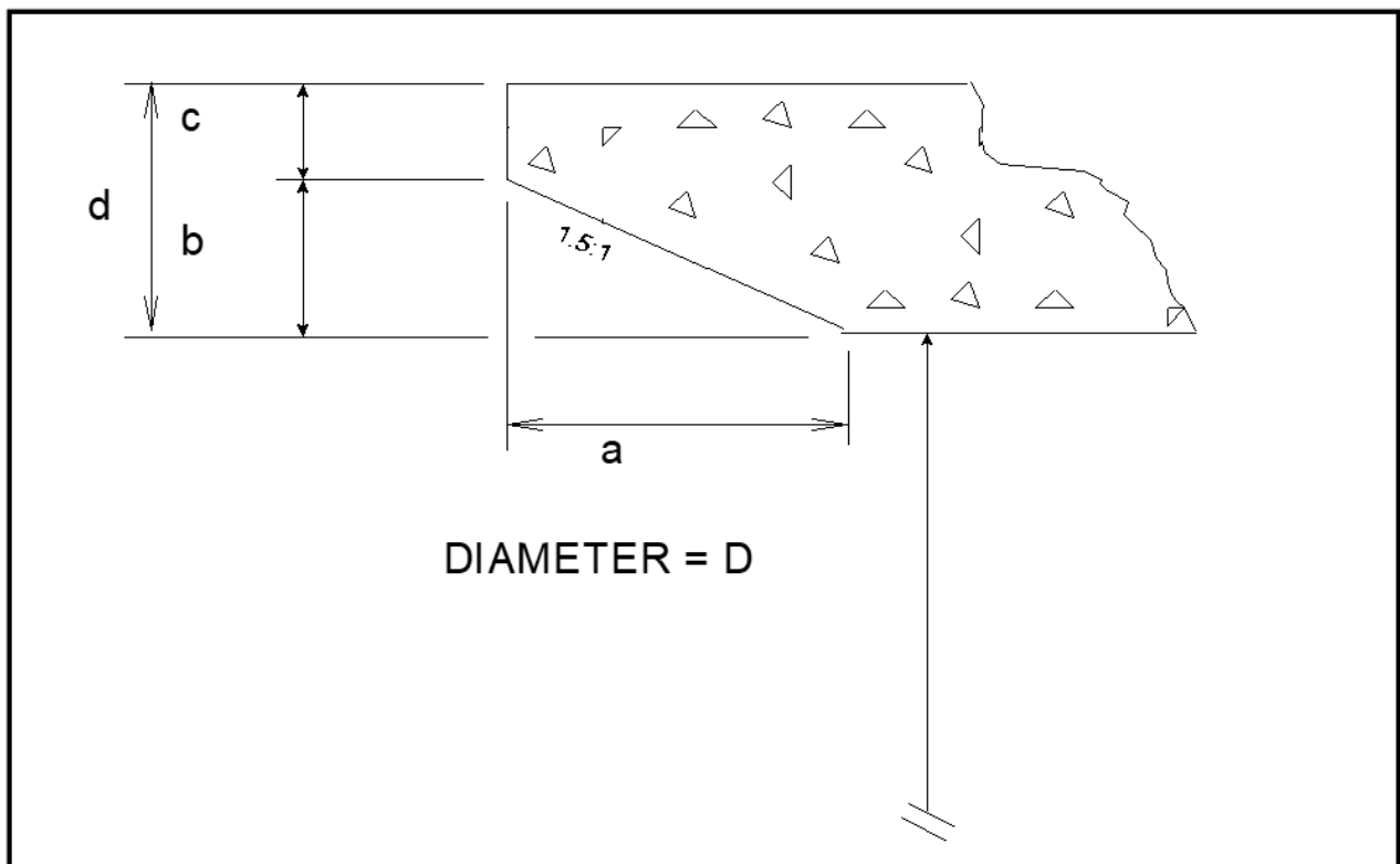
Culvert Inlet with Beveled Ring Entrance
