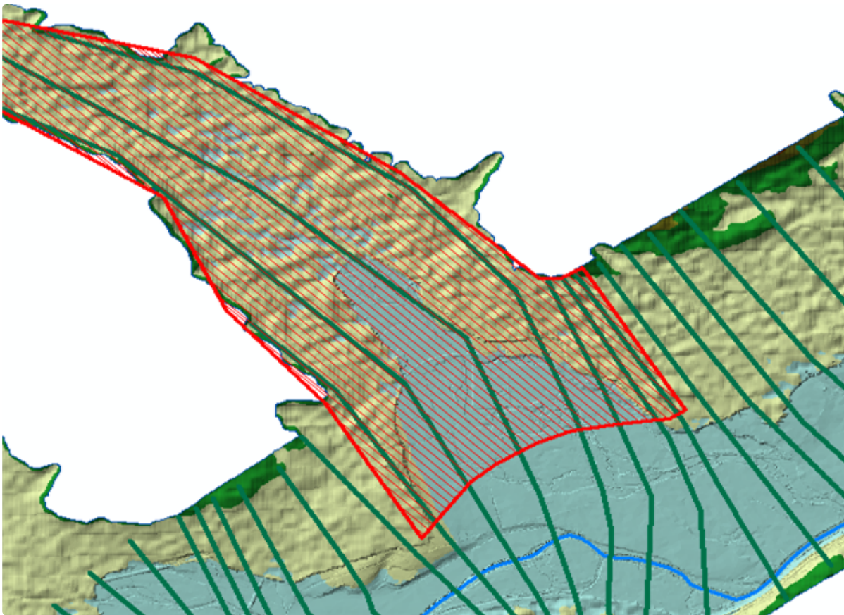
Tributary storage modeled as cross section ineffective flow areas.
