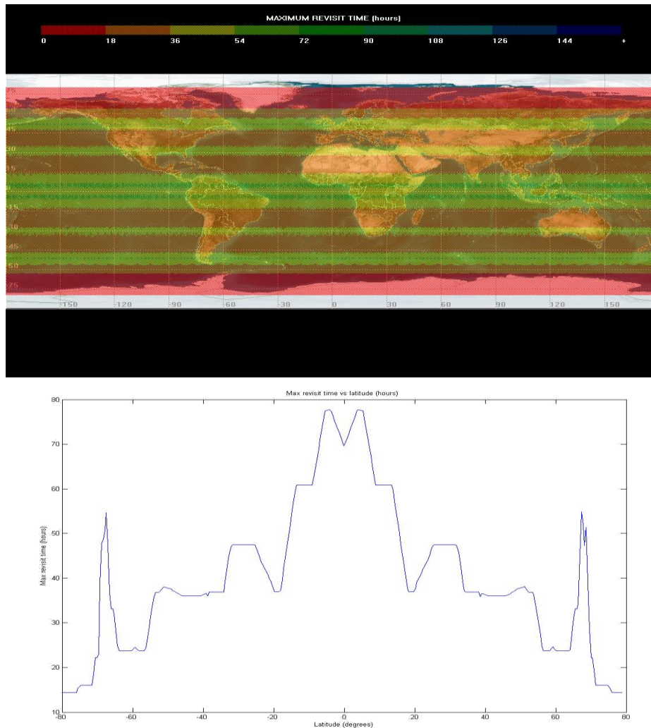
Figure 9 – PAZ revisit times
