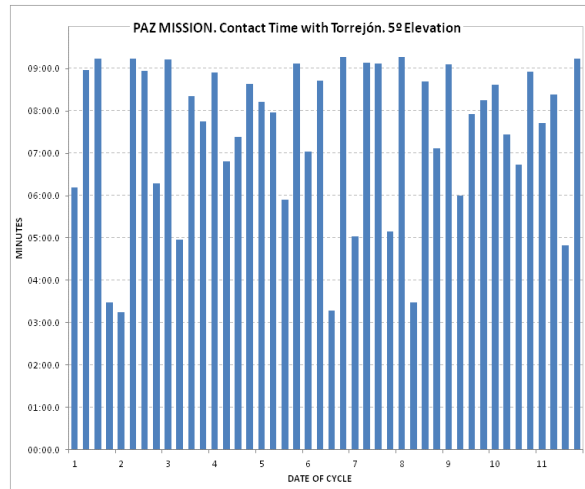
Figure 10 - Distribution of contact time with Torrejón station in one cycle
