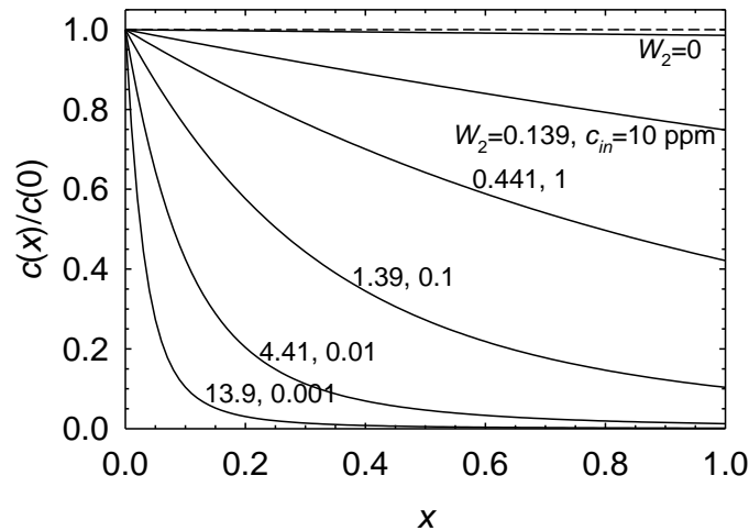
Figure 3.5.4. Dimensionless SO 2 contaminant concentration in the gas phase (equation 3.5.7) as a function of the dimensionless flow field channel length x and parameter W_2 . W_1=0.0145 . Reprinted and reformatted with permission from ECS Trans. , 50 (2), 649 (2012). Copyright 2012, The Electrochemical Society.
