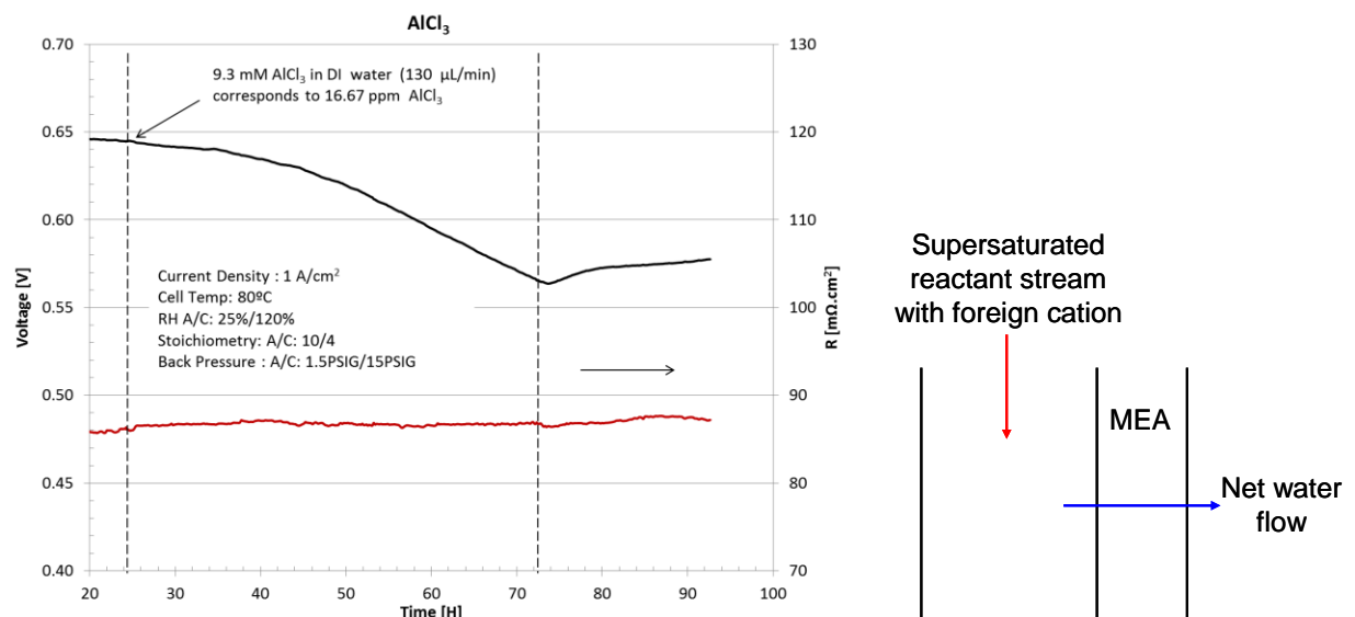
Figure 2.1.6. Cell voltage and resistance transients resulting from Al 3+ contamination (left). Conceptual approach to favor the transport of foreign cations toward the ionomer and membrane (right). Left figure, reformatted original, Journal of The Electrochemical Society , 162 (4) F373-F379 (2015). © The Author(s) 2015. Published by ECS. This is an open access article distributed under the terms of the Creative Commons Attribution Non-Commercial No Derivatives 4.0 License (CC BY-NC-ND, http://creativecommons.org/licenses/by-nc-nd/4.0/ ), which permits non-commercial reuse, distribution, and reproduction in any medium, provided the original work is not changed in any way and is properly cited. For permission for commercial reuse, please email: oa@electrochem.org. [DOI: 10.1149/2.0291504jes]. All rights reserved.
