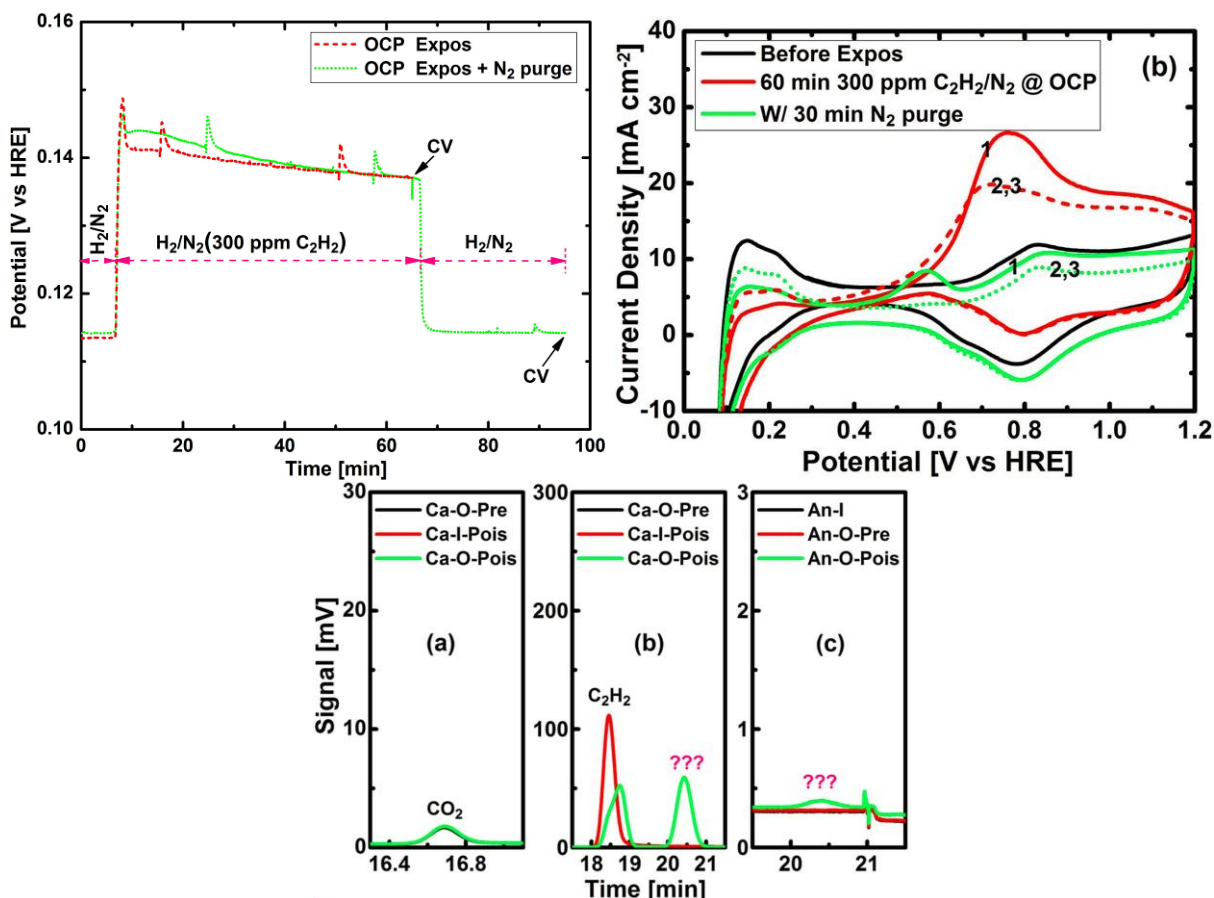
Figure 2.3.21. Chronopotentiometric transients (top, left) and cyclic voltammograms (top, right) for a fuel cell exposed to a mixture of \text{C}_2\text{H}_2 in \text{N}_2 at OCP. Gas chromatographs for a fuel cell fed with a mixture of \text{C}_2\text{H}_2 in \text{N}_2 at OCP (bottom).
