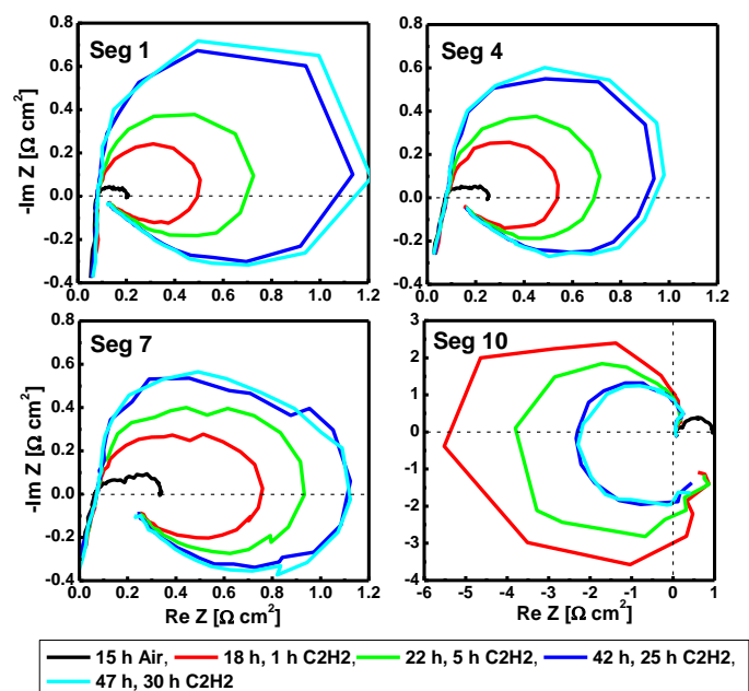
Figure 2.3.16. Local impedance spectra obtained before and during contamination by 300 ppm C 2 H 2 . Air baseline and after shorter and longer contaminant exposure periods. 1 A cm -2 .
