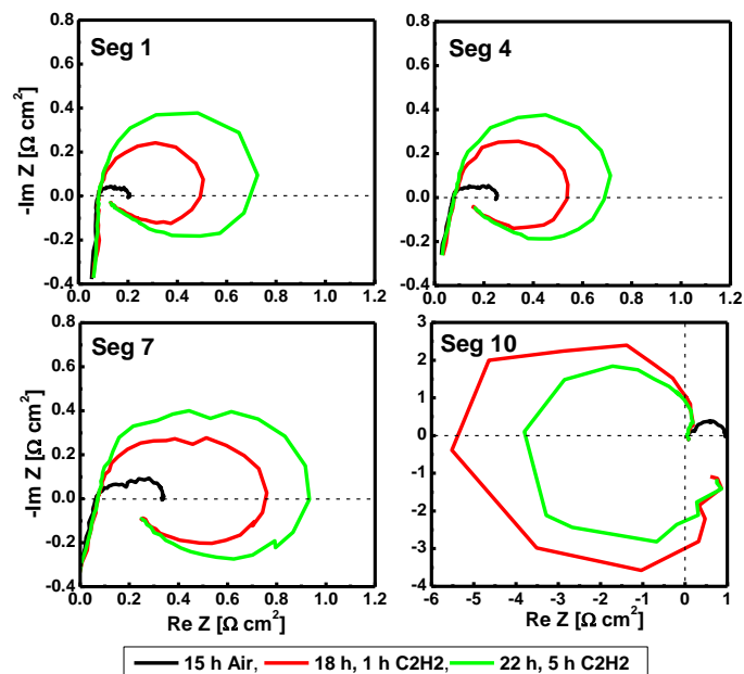
Figure 2.3.15. Local impedance spectra obtained before and during contamination by 300 ppm C 2 H 2 . Air baseline and after shorter contaminant exposure periods. 1 A cm -2 .
