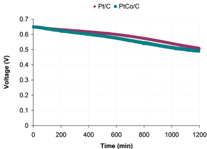
Figure 2.6.3. Comparison between single cell performance transients resulting from the injection of 134 ppb SO 2 in air for a Pt and a PtCo catalyst. 75 °C, 1.5 A cm -2 , 21.6 psig, 100 % relative humidity, air stoichiometry of 4, 20 h SO 2 exposure, 45 cm 2 active area, 0.4/0.1 mg Pt cm -2 for the cathode/anode.
