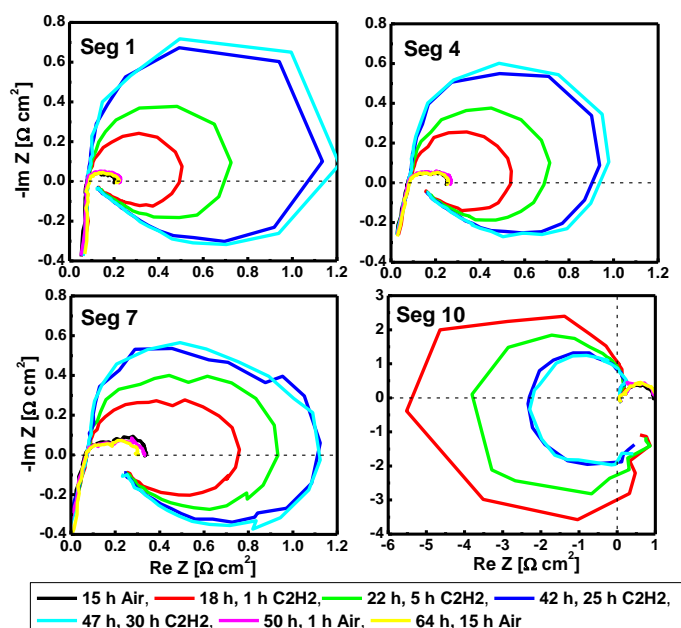
Figure 2.3.17. Local impedance spectra obtained before, during, and after contamination by 300 ppm C_2H_2 . Air baseline and after contaminant exposure and recovery periods. 1 A cm^{-2} .
