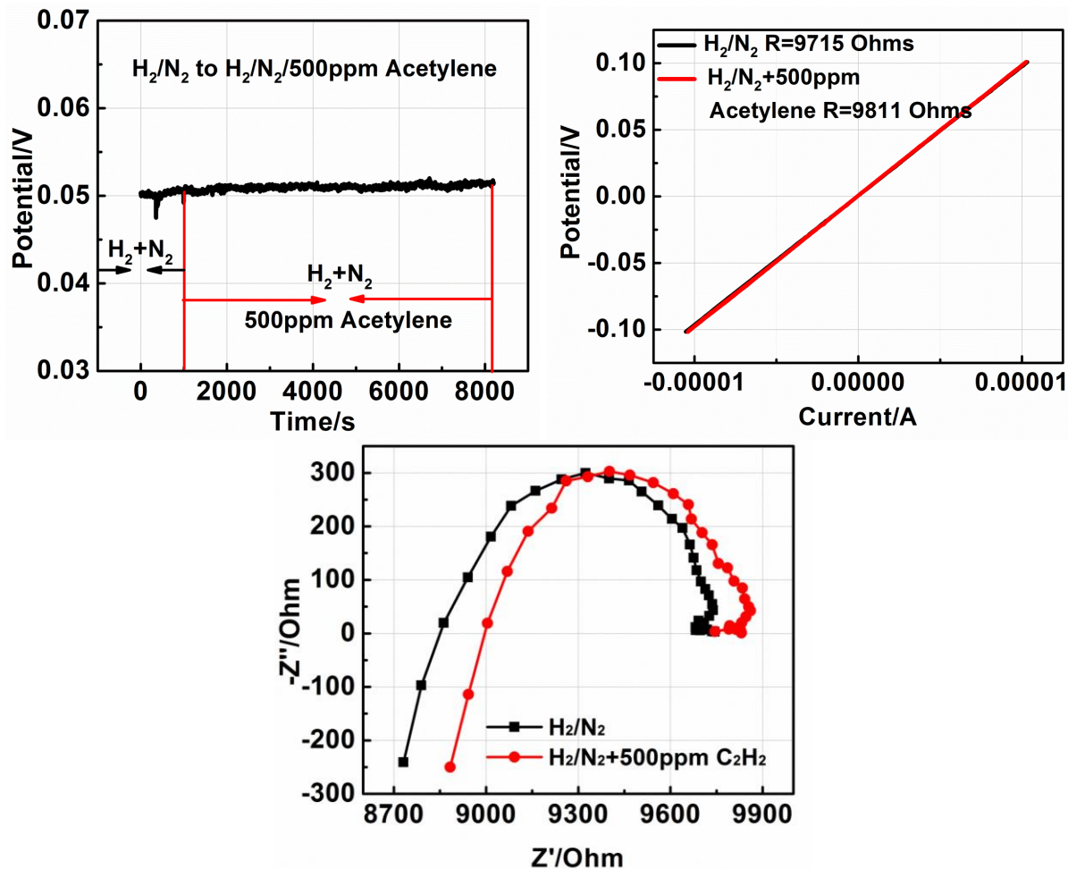
Figure 2.3.13. Nafion XL membrane conductivity measurements in a BektTech cell flowing a mixture of H_2/N_2 without or with 500 ppm C_2H_2 . Measurements were completed by chronopotentiometry (top, left), cyclic voltammetry (top, right) and impedance spectroscopy (bottom).
