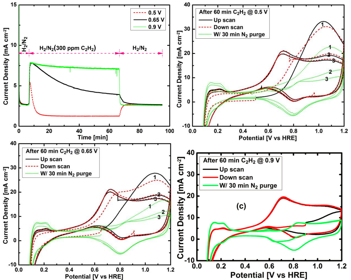
Figure 2.3.22. Chronopotentiometric transients (top, left) and cyclic voltammograms for a fuel cell exposed to a mixture of C 2 H 2 in N 2 at 0.5 V (top, right), 0.65 V (bottom, left) and 0.9 V (bottom, right).
