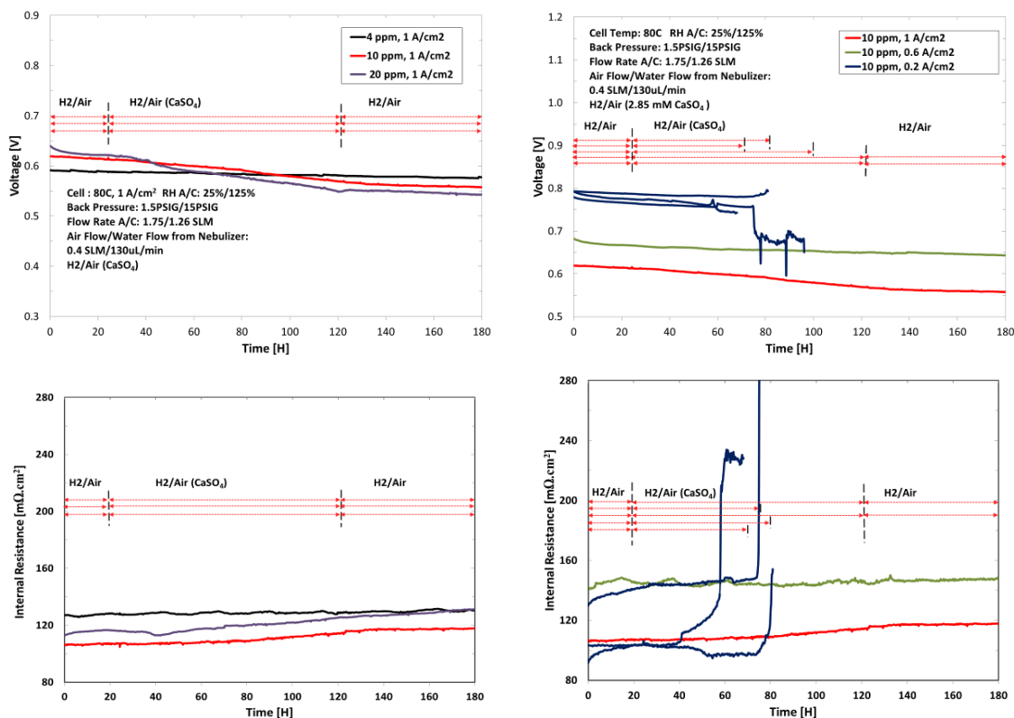
Figure 2.2.6. Effect of contaminant concentration (left) and current density (right) on cell voltage (top) and cell resistance (bottom) for a fuel cell temporarily contaminated with Ca 2+ . Reprinted and reformatted with permission from ECS Trans. , 58 (1), 529 (2013). Copyright 2013, The Electrochemical Society.
