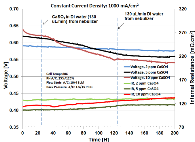
Figure 2.3.33. Effect of contaminant concentration on cell voltage and cell resistance for a fuel cell temporarily contaminated with Ca^{2+} (replotted data from figure 2.2.6, top and bottom, left). Reprinted and reformatted with permission from ECS Trans. , 58 (1), 529 (2013). Copyright 2013, The Electrochemical Society.
