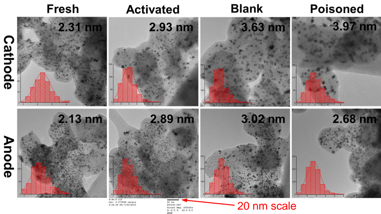
Figure 2.4.7. High resolution transmission electron microscopy pictures of cathode and anode catalysts after different operation condition sets.
