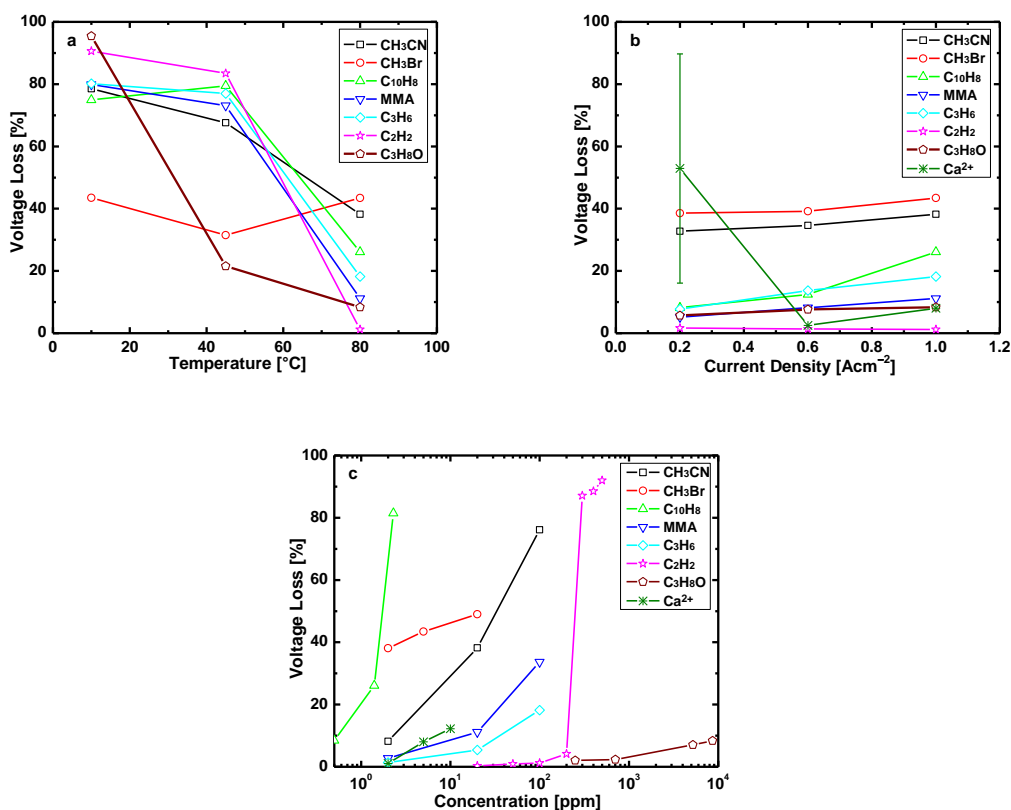
Figure 2.2.8. Effect of temperature (top, left), current density (top, right) and contaminant concentration (bottom) on fuel cell performance losses for 7 airborne contaminants and a foreign cation. CH 3 CN: acetonitrile, CH 3 Br: bromomethane, C 10 H 8 : naphthalene, MMA: methyl methacrylate, C 3 H 6 : propylene, C 2 H 2 : acetylene, C 3 H 8 O: iso-propanol, Ca 2+ : calcium.
