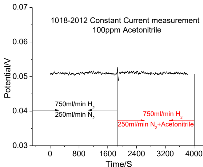
Figure 2.3.26. Nafion XL membrane conductivity measurements in a BektTech cell flowing a mixture of H_2/N_2 without or with 100 ppm CH_3CN . Measurements were completed by chronopotentiometry.
