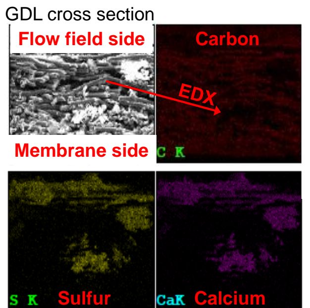
Figure 2.3.28. Photographs of the cathode flow field plate and gas diffusion electrode after contamination by \text{Ca}^{2+} (top). Scanning electron microscopy and energy dispersive X-ray spectroscopy of the white deposits on the gas diffusion layer surface indicate the presence of \text{CaSO}_4 crystals. Similar tests completed with a cross section of the gas diffusion layer also revealed \text{CaSO}_4 crystals within the structure (bottom). The top figure is reprinted and reformatted with permission from J. Electrochem. Soc. , 161 , F1006 (2014). Copyright 2014, The Electrochemical Society.
