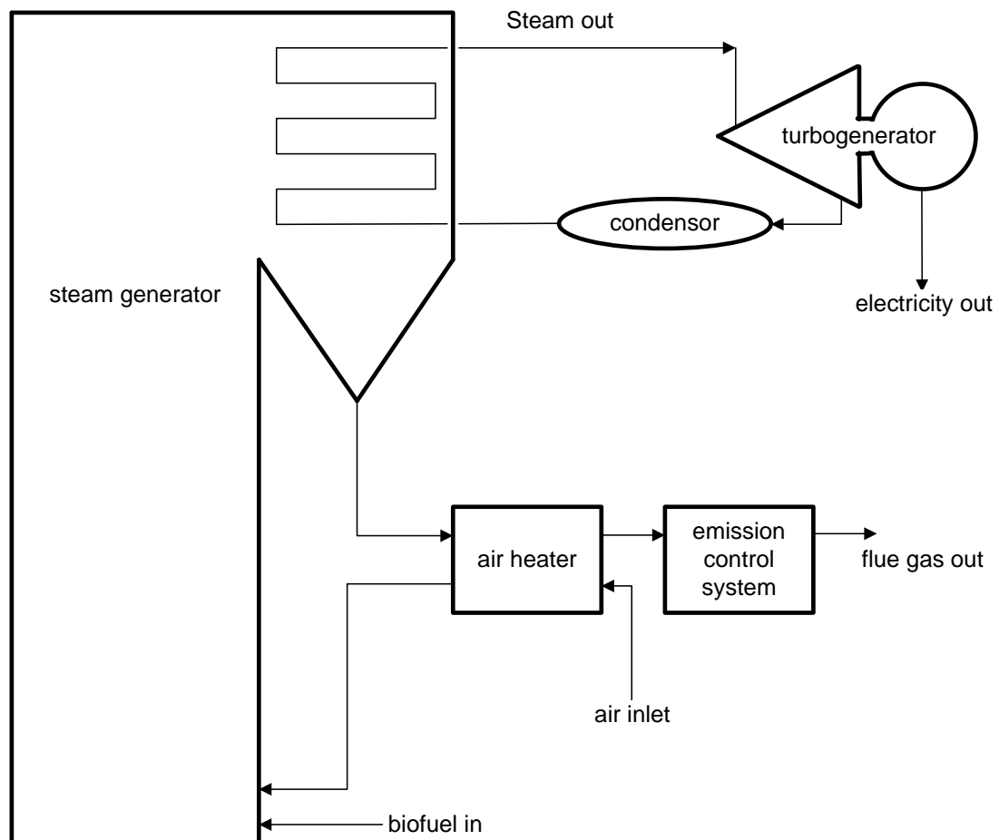
Figure 13. Schematic of direct combustion system
