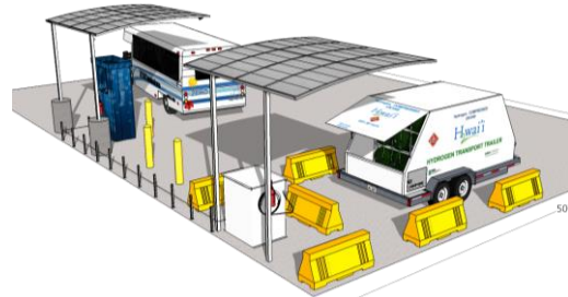
Figure 11. Concept design of MTA fueling dispensing station.
