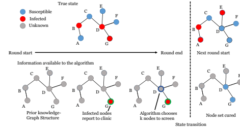
Figure 2: The procedure of the ACTS problem.
