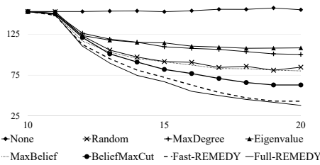
Figure 3: The average number of infected nodes (y-axis) vs. time (x-axis) of the ACTS stage in the India network.
