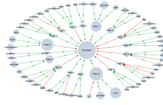
Figure 2: GAF (with attacks -; supports +) for a text classifier.
