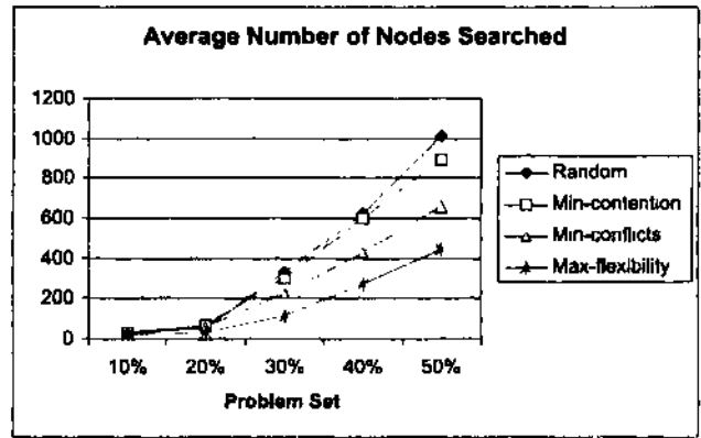
Figure 6: Search Nodes Explored
