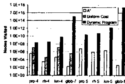
Figure 2: Effectiveness of the factored A^* bound for the multiple alignment of several sequence sets. Numbers in the data set names give the number of sequences being aligned. Note the log scale: for example, on glob-7 the A^* search is over a trillion times more efficient than exhaustive search.
