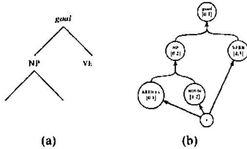
Figure 4: Two representations of a parse: (a) a tree, (b) a path in the edge hypergraph.
