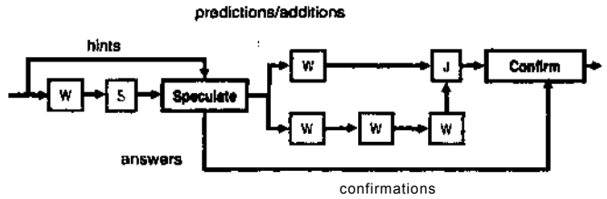
Figure 7: Augmented plan for speculative execution
