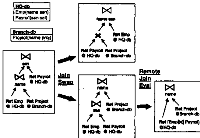
Figure 5: Planning by Rewriting searches through the space of possible transformations on a plan
