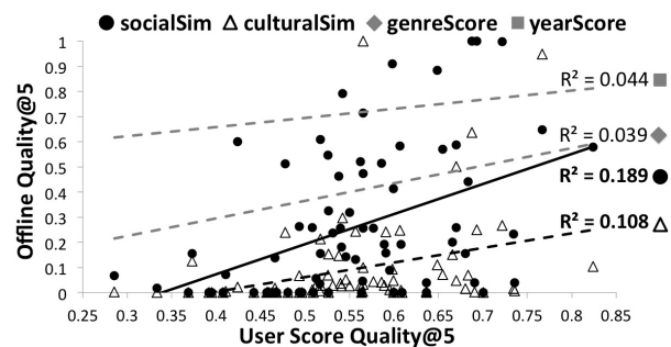
Figure 8: Comparison of User and System-Centric Scores
