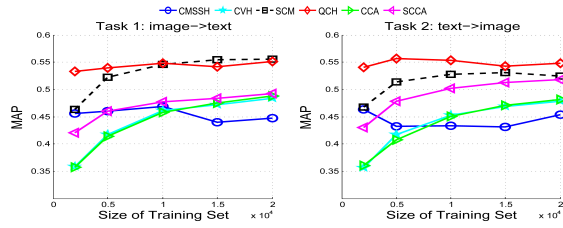
Figure 3: MAP results of different algorithms for two tasks on NUS-WIDE dataset with various numbers of training data.
