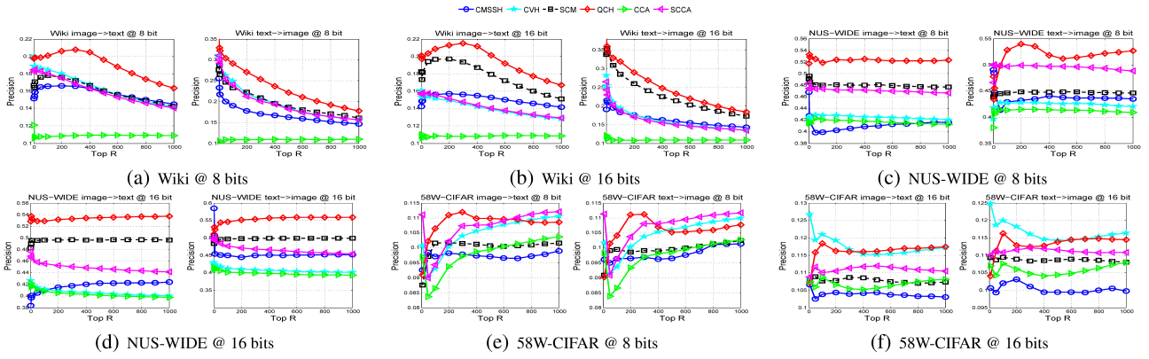
Figure 4: Precision results of different algorithms for two tasks with R varying from 50 to 1000 on the condition of two kinds of bit lengths: 8 bits (4(a) Wiki, 4(c) NUS-WIDE, and 4(e) 58W-CIFAR) and 16 bits (4(b) Wiki, 4(d) NUS-WIDE, and 4(f) 58W-CIFAR), respectively.
