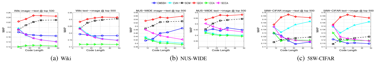
Figure 6: MAP results of different algorithms with various code lengths for two tasks on the three datasets (6(a) Wiki, 6(b) NUS-WIDE, and 6(c) 58W-CIFAR).
