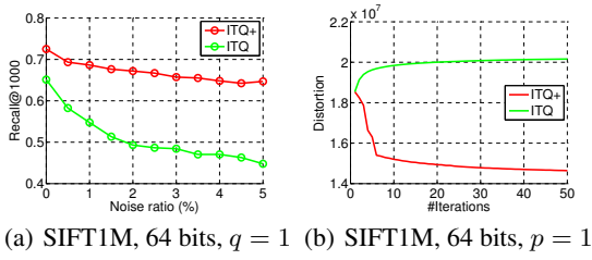
Figure 1: ITQ does not perform well with the noisy data (left) and can not deal with some other similarity measures (right).
