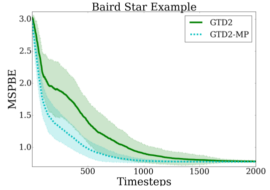
Figure 1: Off-Policy Convergence Comparison
