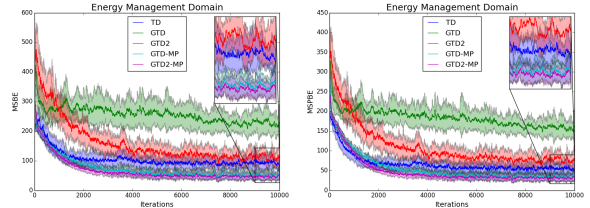
Figure 2: Energy Management Example
