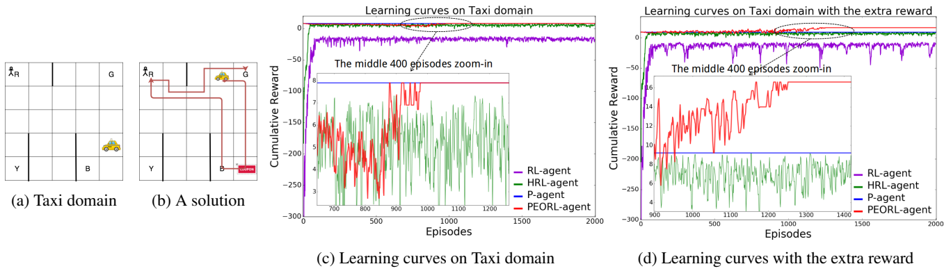
Figure 2: Taxi domain
