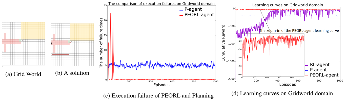
Figure 3: Grid World
