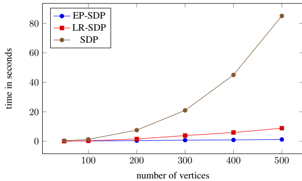
Figure 3: Time complexity
