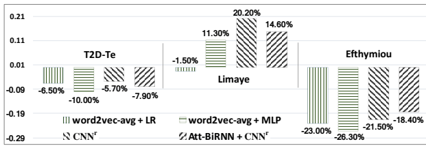
Figure 2: Accuracy improvement using surrounding columns. Cells of surrounding column are appended to the main cell through vector concatenation (word2vec-avg + LR and word2vec-avg + MLP) and row feature learning (CNN and Att-BiRNN + CNN).
