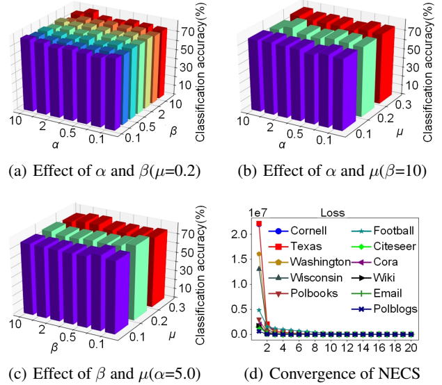
Figure 3: Parameter sensitivity and convergence.
