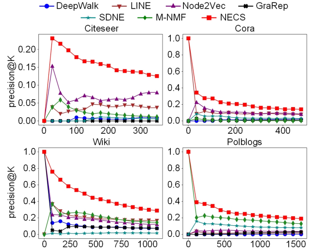
Figure 2: Link prediction results in terms of precision@K .
