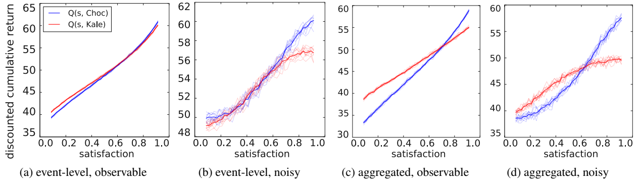
Figure 2: Q-values as a function of satisfaction level in the Choc-Kale model. Model parameters: \beta = 0.9, \tau = 0.25, \mu_{\text{Choc}} = 8, \mu_{\text{Kale}} = 2, \sigma_{\text{Choc}} = \sigma_{\text{Kale}} = 0.5 . Observations (satisfaction s ) are corrupted with additive Gaussian noise (mean 0, stddev. 0.3) truncated on [-1, 1] .
