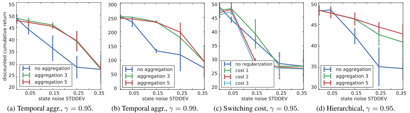
Figure 3: Experimental results. Cumulative discounted returns of event-level, aggregated and regularized policies on the Choc-Kale POMDP.
