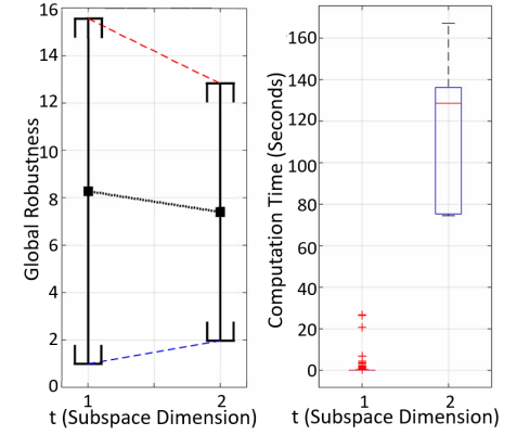
Figure 2: Robustness evaluation of DNN-0 for t \in \{1, 2\} and box-plots of computation time.
