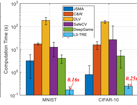
Figure 6: Means and standard deviations of computational time of all methods.
