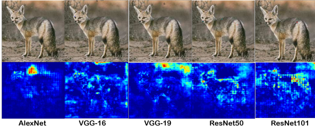
Figure 8: Adversarial examples on upper boundaries (top) and saliency maps (bottom).
