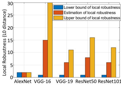
Figure 9: Lower bounds, upper bounds and estimates of local robustness for 5 ImageNet DNNs on a given image.
