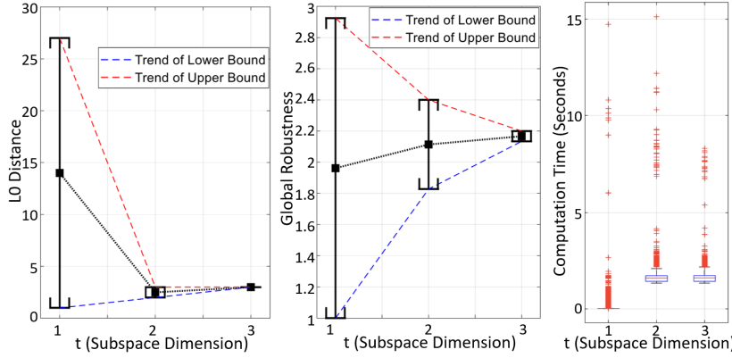
Figure 1: (Left) Convergence of lower bound, upper bound, and estimation of d_m for one image; (Middle) That of global robustness; (Right) Boxplots of computation time.
