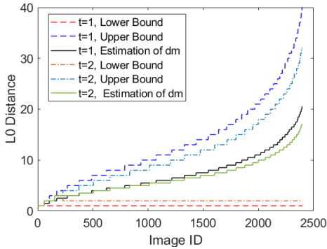
Figure 4: DNN-0: Upper bounds, lower bounds, and estimations of d_m for all sampled input images for t \in \{1, 2\} .
