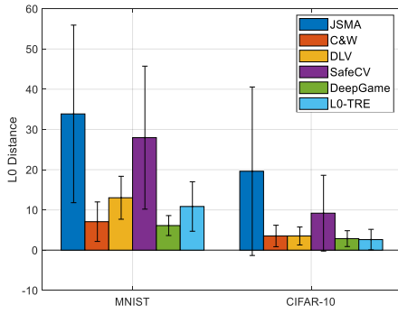
Figure 5: Means and standard deviations of the adversarial L_0 distance.
