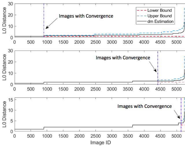
Figure 3: sDNN: Upper bounds, lower bounds, estimations of d_m for all sampled images for t \in \{1, 2, 3\} ordered from the top to bottom.
