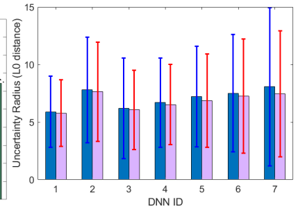
Figure 11: Means and standard deviations of uncertainty radius d_m for 1,000 test images at t = 1, 2 .
