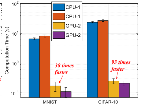
Figure 7: Means and standard deviations of computational time with CPUs or GPUs.
