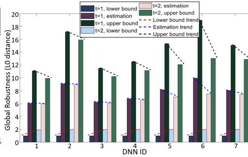
Figure 10: Lower bounds, upper bounds, and global robustness estimates for t \in \{1, 2\} for seven DNN models.
