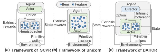
Figure 1: Illustration of policy learning frameworks for CRS, including a framework of the outsourcing strategy (SCPR), a unified framework (Unicorn), and our proposed Director-Actor framework.
