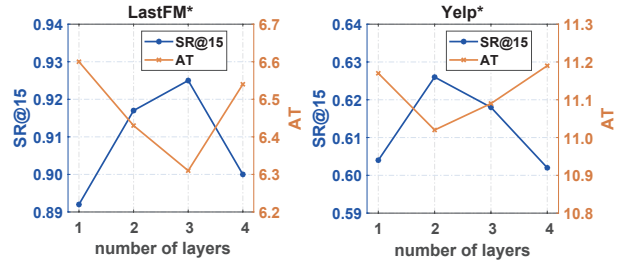
Figure 4: Impact of Layer Number(L)
