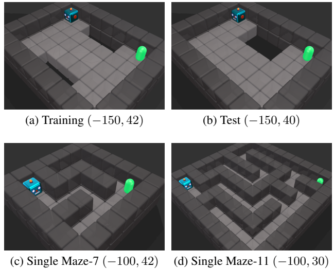
Figure 2: Evaluation environments : Holey distributional shift gridworlds inspired by [Leike et al. , 2017] for training (Figure 2a) and shifted evaluation (Figure 2b), as well as deterministic configurations of Maze 7 (Figure 2c) and Maze11 (Figure 2d) inspired by [Cobbe et al. , 2020]. The agents’ goal is to reach the target (green capsule), rewarded with 50. To incentivize the shortest path, every step is penalized with -1 . Holes immediately terminate the episode and are penalized with -50 . Episodes are terminated after a maximum of 100 steps. Sub-captions show the name and return ranges.
