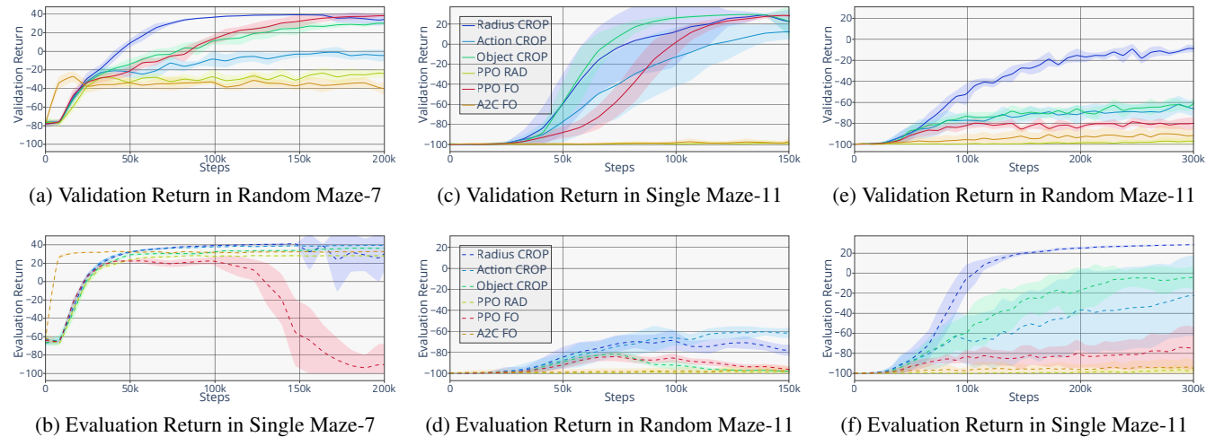
Figure 4: Generalization Benchmark: Comparing R-CROP (blue), A-CROP (light blue), O-CROP (green), RAD (yellow) and FO (red) for training PPO, and A2C using FO (orange) in 100 random Maze-7, a single Maze-11, and 100 random Maze-11 configurations for 200k, 150k, and 300k steps (x-axis) respectively, w.r.t. the Validation Return (solid lines in Figure 4a, Figure 4c, and Figure 4e) and the Evaluation Return (dashed lines in Figure 4b, Figure 4d, and Figure 4f) on the y-axis, averaged over eight random seeds. The shaded areas mark the 95% confidence intervals.
