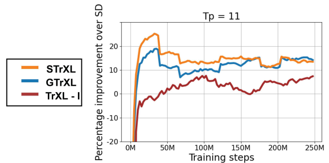
Figure 10: RL Training progression for ht=2m angle=30° for STrXL, GTrXL, and TrXL-I function approximators.
