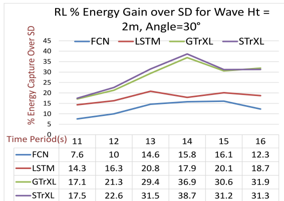
Figure 7: % Increase of Energy Capture over SD controller for 30° waves for Height=2m with different Function Approximations.
