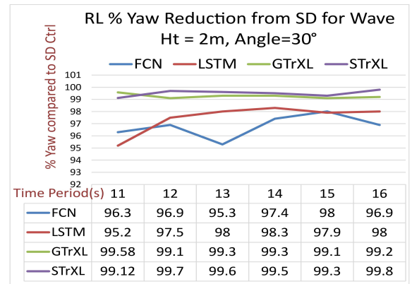
Figure 8: % Yaw Reduction over SD controller for 30° waves for Height=2m with different Function Approximations.
