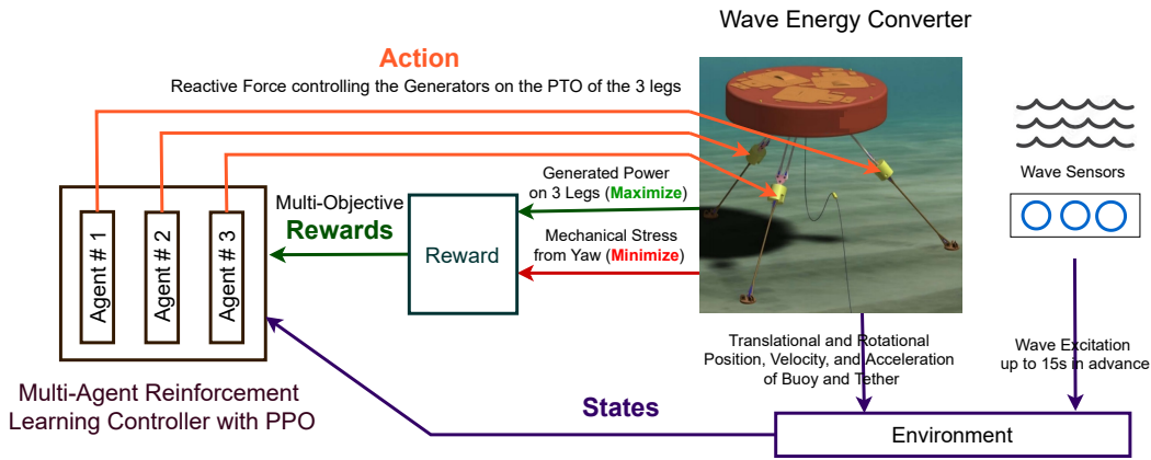
Figure 4: Architecture of Multi-Agent RL controlling the WEC
