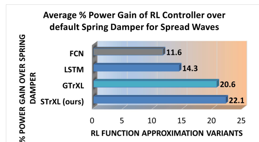
Figure 1: Average Power Gain of RL Controller for different Function Approximations over default Spring Damper Controller
