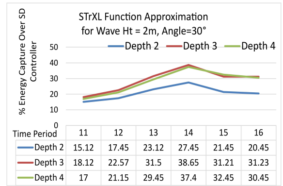
Figure 9: % Increase of Energy Capture over SD controller for 30° waves for Height=2m with STrXL with a variation of a number of layers or depth.
