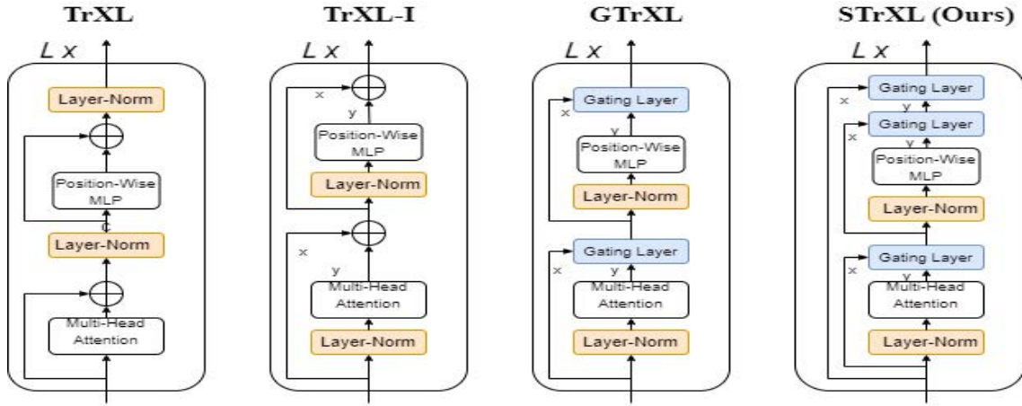
Figure 6: Variations of Transformer blocks to facilitate convergence. The overall architecture has L such blocks. TrXL : A traditional transformer with multi-head attention and layer normalization, TrXL-I : The layer norm is included with the input stream, GTrXL : Includes a gating layer to include the residual connection around the attention and MLP blocks ([Parisotto et al. , 2020]), STrXL : Residual connections with gating layer around the transformer block.
