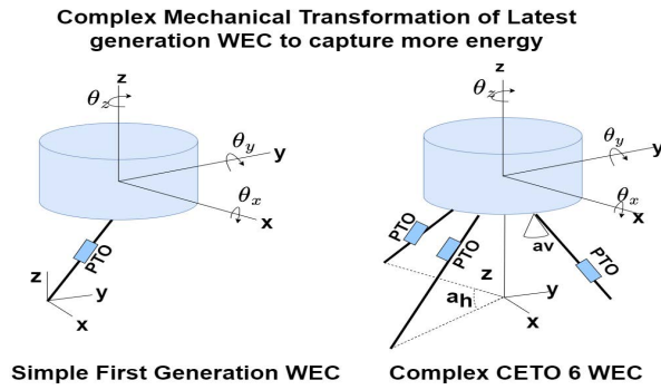
Figure 2: Increase in the structural complexity from 1-tether to the 3-tether WEC to capture more power with 6 degrees of translational and rotational motions. [Rijnsdorp et al. , 2018]
