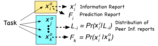
Figure 4: Bayesian Truth Serum: Agent A_i observes the information in yellow; it is scored against the information from others (blue).
