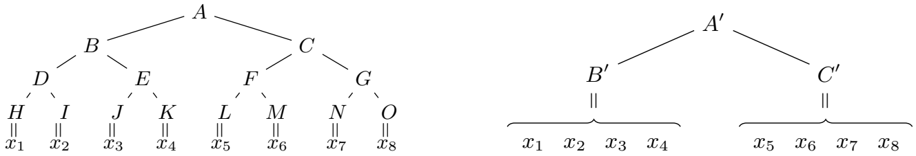
Figure 2: Totalizer representation of 2x_1 + 3x_2 + 4x_3 + 5x_4 + 3x_5 + 4x_6 + 6x_7 + 8x_8 \leq 10 (left) and, of (2x_1 + 3x_2 + 4x_3 + 5x_4 + 3x_5 + 4x_6 + 6x_7 + 8x_8 \leq 10, \{\{x_1, x_2, x_3, x_4\}, \{x_5, x_6, x_7, x_8\}\}) (right).
