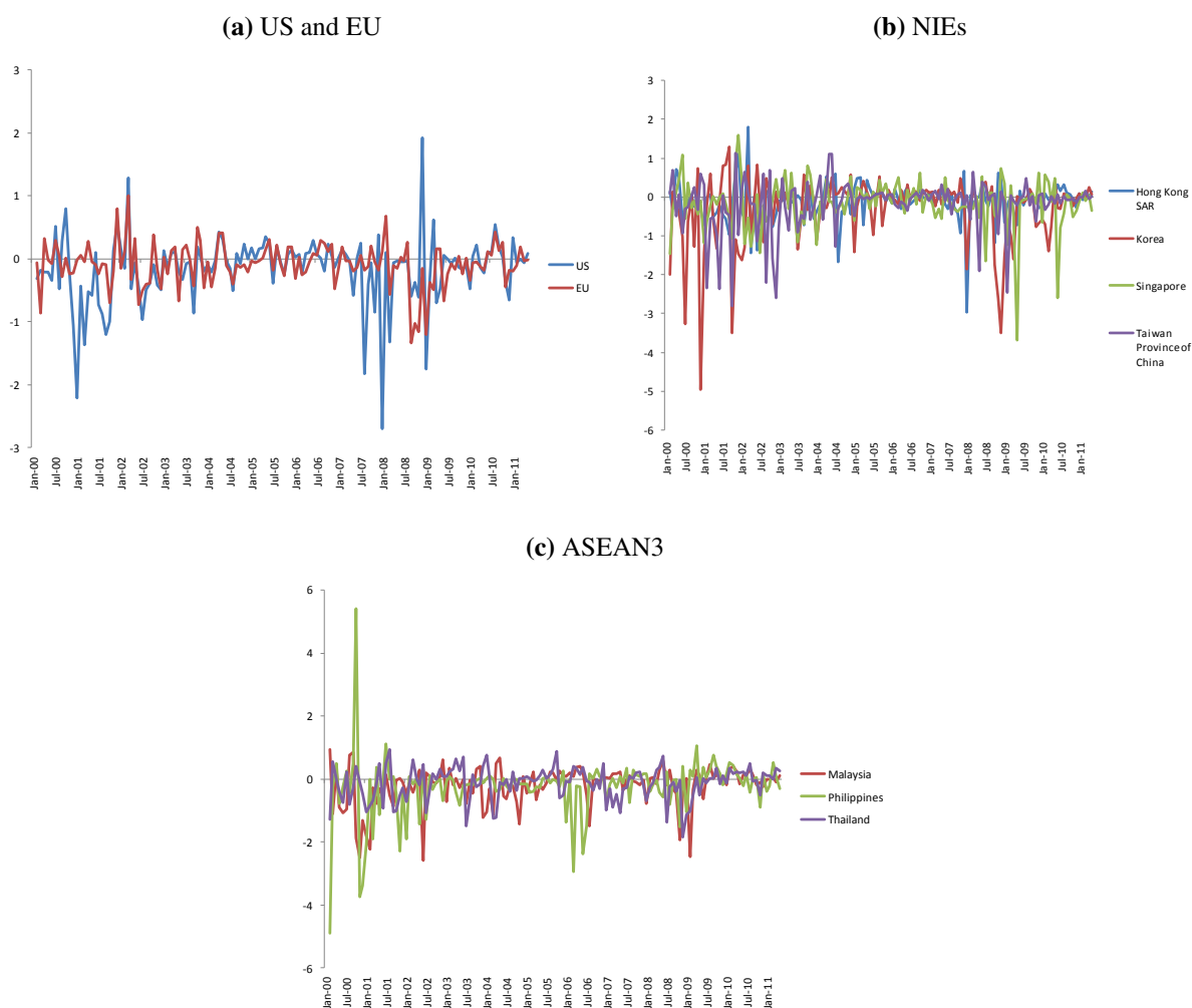
Figure 1: Log Stochastic Discount Factors
