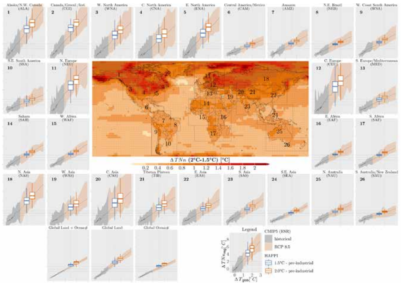
Figure 3.SM.8 | Same analysis as Figure 3.5, but for the annual minimum value of daily minimum temperature (Tn). For more details on computation, see description of computation of Figure 3.5 in the present Annex, as well as Wartenburger et al. (2017), Seneviratne et al. (2016) and Seneviratne et al. (2018).
