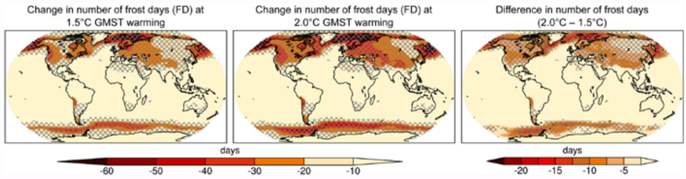
Figure 3.SM.13 | Projected changes in number of frost days (days with T < 0^{\circ}\text{C} , bottom) at 1.5°C (left) and 2°C (middle) GMST increase, and their difference (right). Cross-hatching highlights areas in which at least 2/3rds of the models agree on the sign of change as a measure of robustness (18 or more out of 26). Adapted from Wartenburger et al. (2017).
