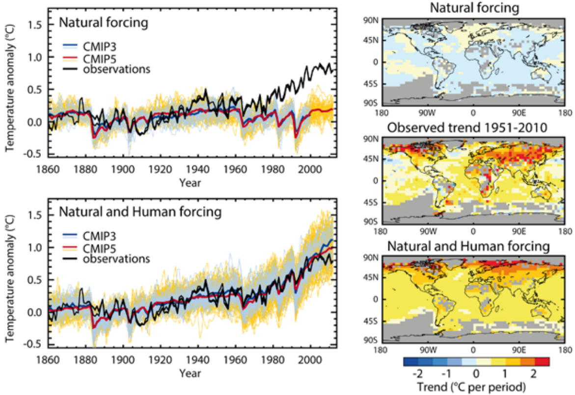
Figure 3.SM.3 | Attribution of global warming change (from IPCC AR5, Bindoff et al., 2013a)
