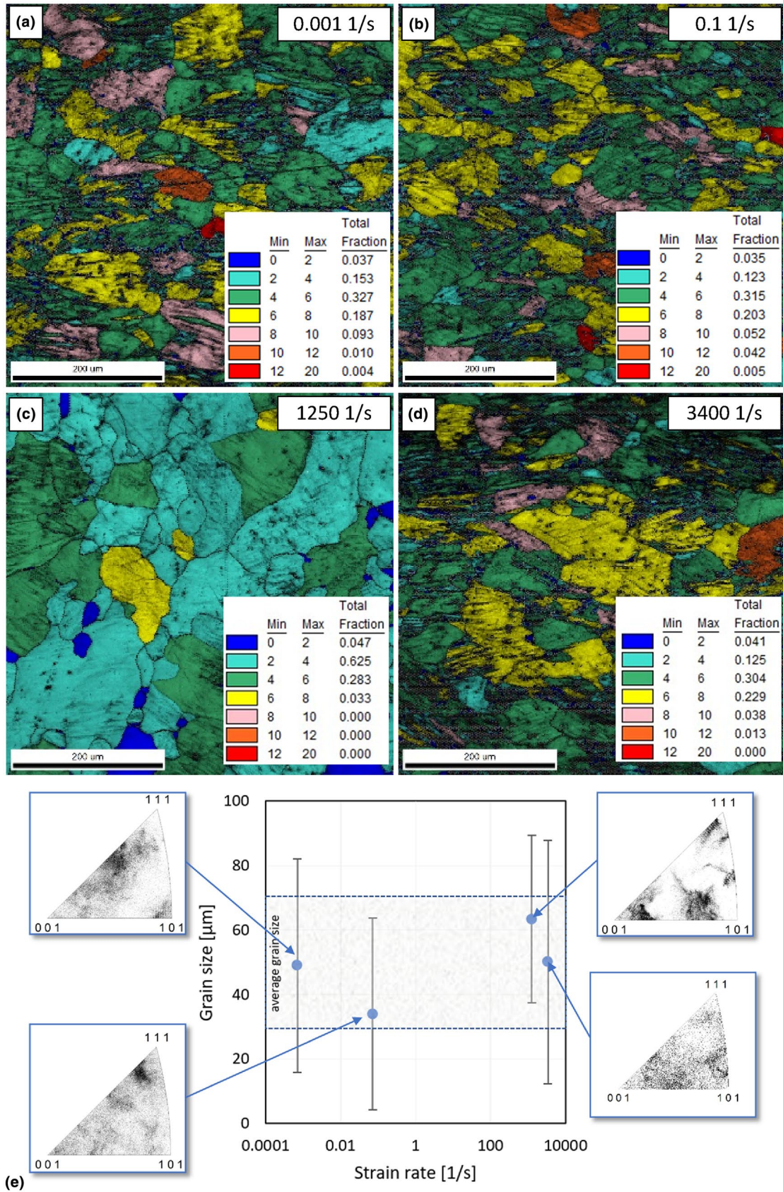
Figure 3. Grain orientation spread after deformation under different values of strain rate: 0.001 1/s (a), 0.1 1/s (b), 1250 1/s (c), 3400 1/s (d); comparison of the average grain size distribution as a function of strain rate at low temperature (e).
