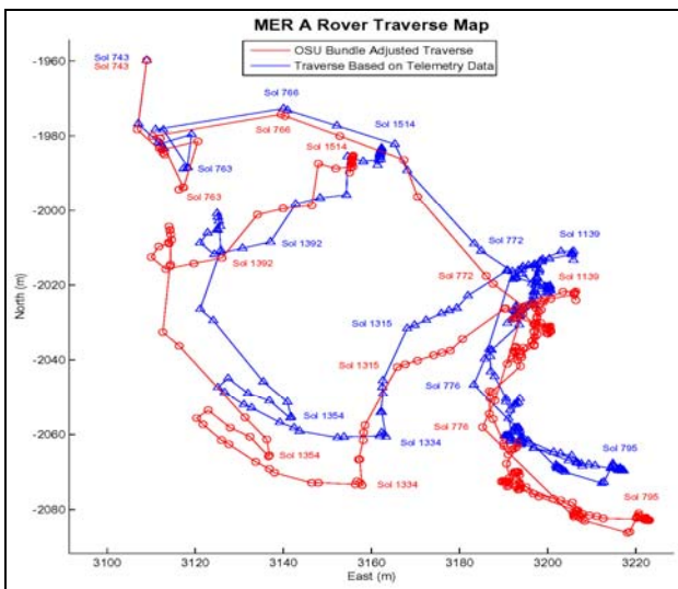
Figure 2. Comparison of Spirit rover traverses in the Home Plate area. Blue line is the traverse computed from telemetry data and red line is the traverse corrected by the bundle adjustment method.
