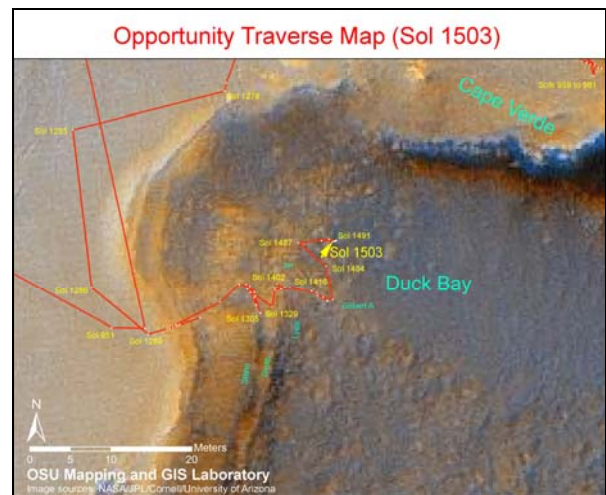
Figure 3. Opportunity rover traverse map at Victoria Crater
