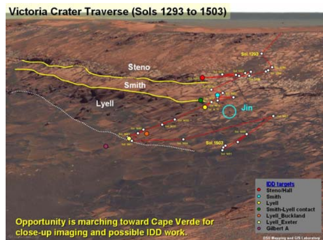
Figure 4. Opportunity rover traverse (red) overlaid on Pancam image mosaic. Small white dots are rover locations. Outcrop layers and target features are marked as lines and larger dots.
