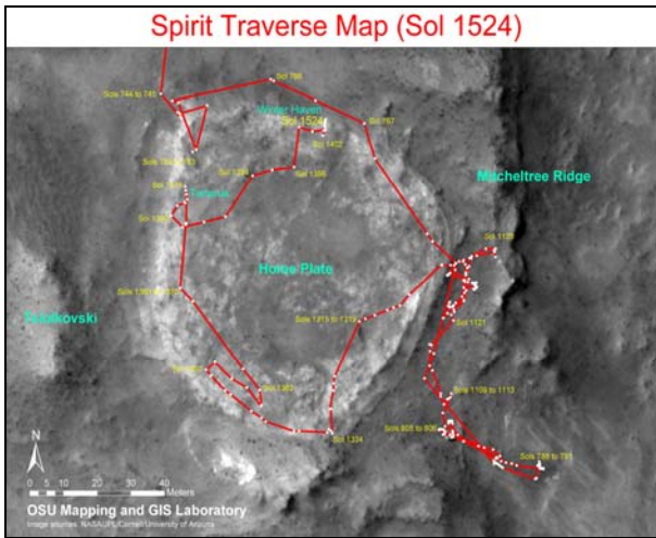
Figure 1. Spirit rover traverse map in the Home Plate area
