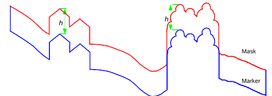
(b) mask and marker ; marker = mask - h except pixels at the boundary of the image when marker = mask
