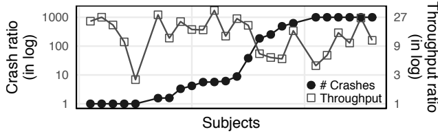
Figure 3: Comparison between distance-based fitness function with and without dynamic PCA in terms of the number of crashes found and test case generation throughput.
