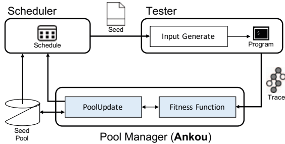
Figure 2: Ankou architecture.
