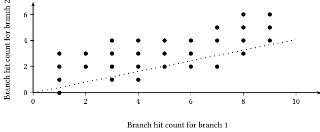
Figure 1: A hypothetical example showing branch-hit-count states of 30 unique program executions. Each dot represents a branch-hit-count state \vec{x} .
