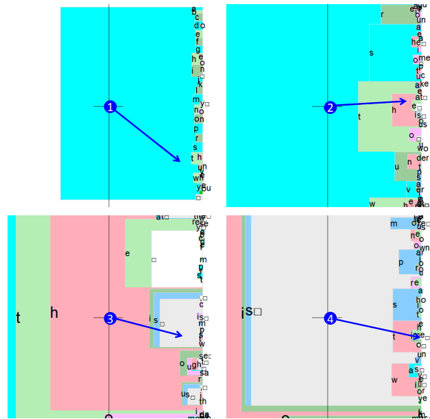
Figure 1: Example of a user writing “this time” in Dasher.
