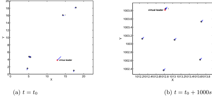
Fig. 1. Flocking of mass point group, N = 6 .
