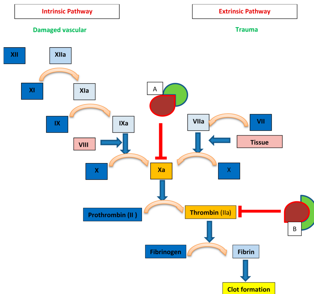
Figure 1. Heparin mechanisms within the coagulation cascade. Box A: AT (red) bound with heparin fragments (green) of any length within the unique pentasaccharide sequence can inhibit factor Xa. Box B: AT (red) bound with heparin (green) with chain length >17 disaccharide units can inhibit thrombin (Factor IIa).
