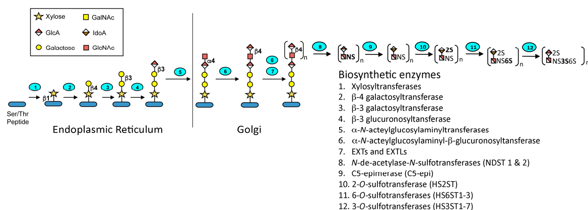
Figure 2. Heparin biosynthesis. The glycosaminoglycan-protein linkage region is first formed under the action of glycosyltransferases. The repeating disaccharide units are then elongated by GlcA and GlcNAc transferases. Chain modifications including N-deacetylation and N-sulfonation, O-sulfonations, and epimerization then occur under the actions of the specified enzymes. Monosaccharide symbols in this figure follow the SNFG (Symbol Nomenclature for Glycans) system [15]
