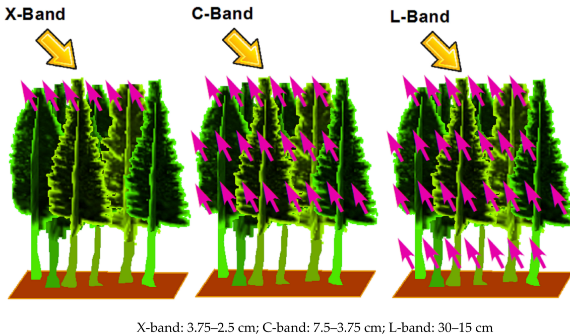
Figure 2. Wavelength illustration of multi-frequency radar system through vegetation. Source: modified from the European Space Agency (ESA).
