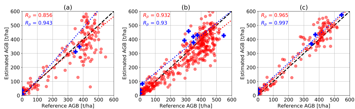
Figure 8. Results for AGB estimation based on (a) heading 124^\circ , (b) heading 275^\circ , (c) both headings combined. Red circles indicate the 200\text{ m} \times 200\text{ m} regions-of-interest (ROIs) using the LiDAR-based AGB map as a reference. Blue crosses indicate the ground measurements. The 1-1 line is indicated by the black dashed line, the blue and red dotted lines show the linear regression for the corresponding reference dataset.
