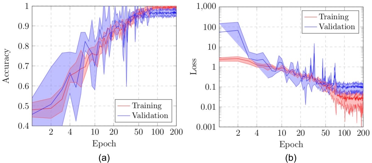
Figure 7: Results of the fourth experiment after 5 independent repetitions. (a) Mean \pm standard deviation training accuracy. (b) Mean \pm standard deviation training loss. In both cases, a logarithmic scale has been set to correctly display the values for a better understanding of the results.
