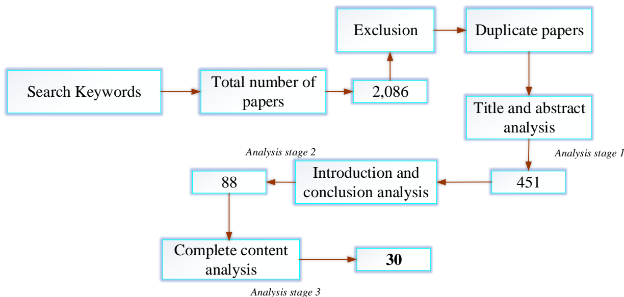
Figure 2: Article selection
