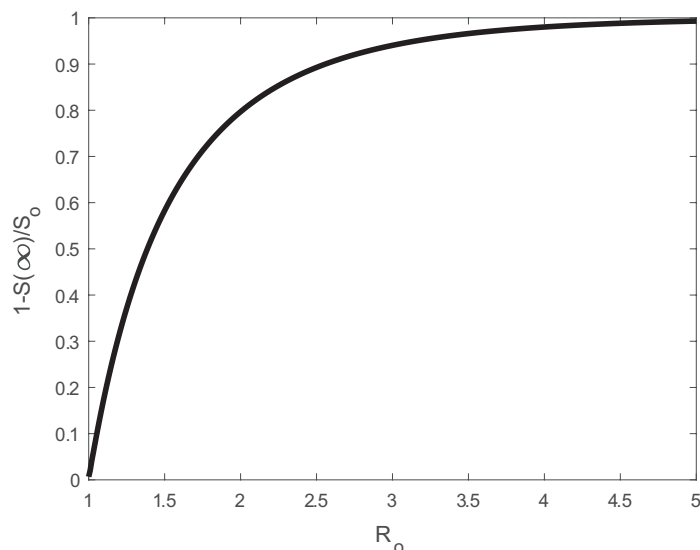
Fig 7. Relation between total infection fraction 1 - S(\infty)/S_o and R_o .
