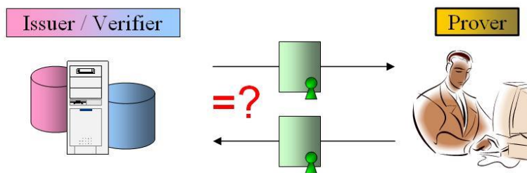
Figure 5: Untraceability property
